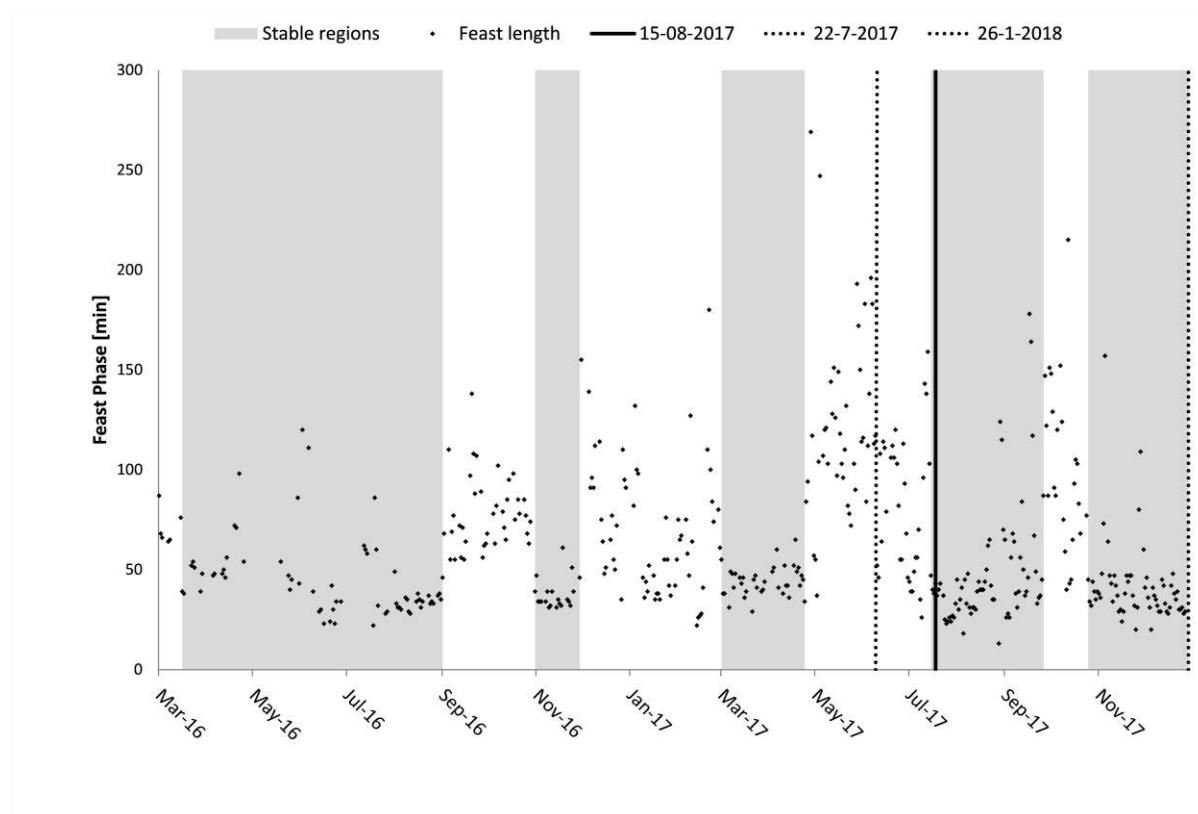
Figure 2. Overview of the performance of the enrichment reactor in terms of the length of the feast phase.
