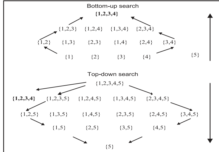
Figure 1: One-Way Searches
