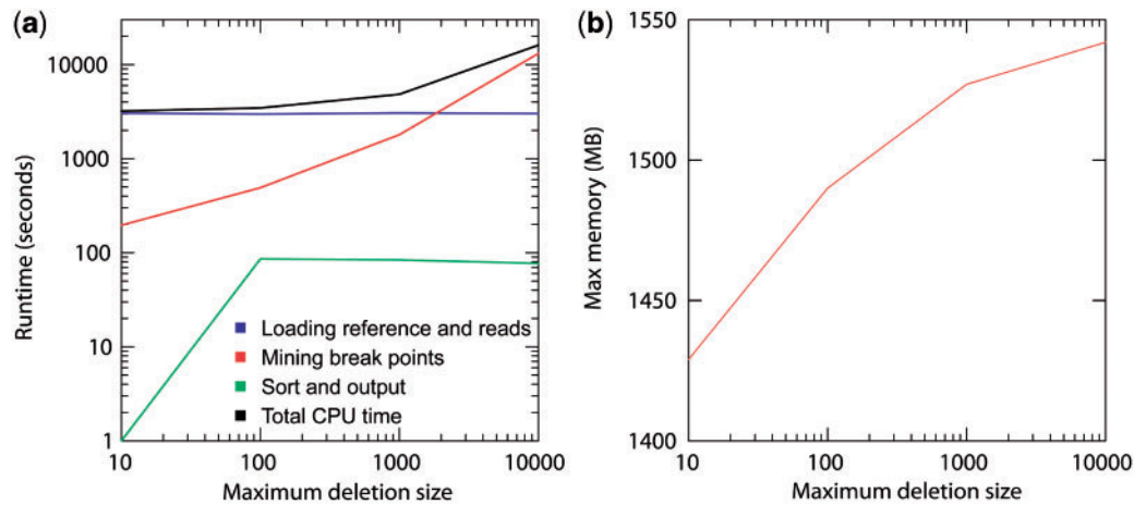
Fig. 6. Runtime and memory consumption for Pindel applied to the NA18507 data on a single CPU for mining indels with different Max_D_Size (10 bp, 100 bp, 1 kb and 10 kb). (a) The user runtime for Pindel is divided into three categories: (i) loading the reference genome and the reads into memory. (ii) Break unmapped reads and map them separately using pattern growth. (iii) Sort break points according to coordinates and write the results on hard disk. (b) Maximum memory consumption for Pindel to process the NA18507 data with different Max_D_Size (10 bp, 100 bp, 1 kb and 10 kb).
