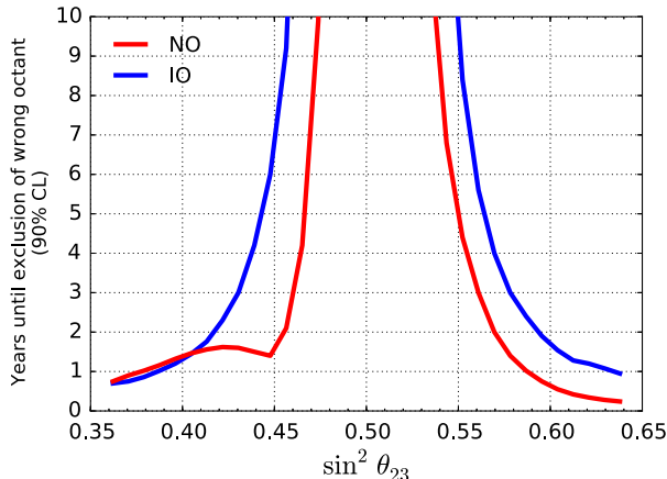
Figure 7: Amount of PINGU data required to determine the \theta_{23} octant (i.e., to exclude the wrong octant at 90% C.L.), as a function of the true mass ordering and true value of \sin^2(\theta_{23}) . Sensitivity is lower if the ordering is inverted as the matter resonance affects antineutrinos rather than neutrinos. The value of \delta_{\text{CP}} has minimal impact and is assumed to be zero.
