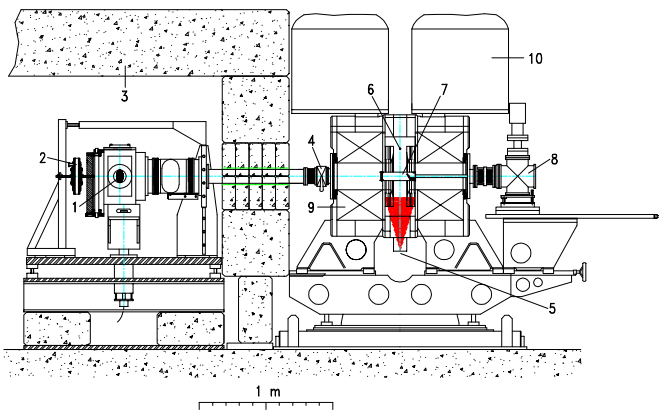
Fig. 4. Sectional drawing of the connection of the cyclotron trap to the crystal chamber of the spectrometer. The symmetry axis of the magnetic field coincides with the line center of the trap to center of the Bragg crystal. 1: Bragg crystal, 2: traction relaxation, 3: concrete shielding, 4: gate valve, 5: X-ray tube (emission cone indicated), 6: position of pion beam without B field, 7: cryogenic target cell including calibration target (right end), 8: target cell support and cryogenic generator, 9: magnet coils of cyclotron trap, 10: LHe dewars.
