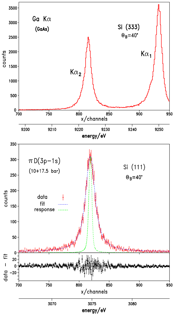
Fig. 8. Top – Ga K\alpha_2 calibration line. The K\alpha_1 component is slightly reduced by the asymmetric emission characteristics of the X-ray tube. Middle – sum spectrum of the \pi D( 3p-1s ) transition measured at the equivalent densities of 10 and 17.5 bar. The narrow structure represents the response function of the crystal spectrometer (normalised to the height of the measured spectrum). Bottom – residuum of data and fit. The fit is performed without assuming any Doppler components.
