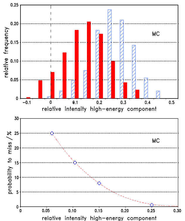
Fig. 10. Top – distributions of relative intensity of a Doppler broadened component induced by the (4 – 3) Coulomb de-excitation transition found from fits to Monte-Carlo (MC) generated spectra. The relative strength used for the simulations is 10% (filled) and 25% (hatched) relative intensity, respectively. In both cases, the result is based on 400 spectra generated for the statistics of the sum of the 10 and 17.5 bar data. Bottom – probability to miss a Doppler contribution corresponding to the (4 – 3) Coulomb de-excitation (modeled by a uniform kinetic energy distribution from (76 – 84) eV) as a function of its relative intensity.
