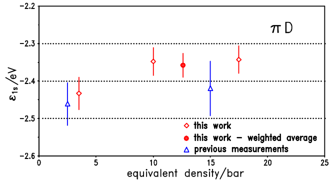
Fig. 12. Experimental information on the hadronic shift in pionic deuterium. The error of the individual measurements at 3.3, 10, and 17.5 bar equivalent density and, therefore, also of the weighted average is dominated by the uncertainty of the Ga K\alpha_2 energy. The results from the two previous experiments at 2.5 bar [45] and 15 bar [44] are adjusted according to the new values for the pure electromagnetic transition energies (Table 7).
