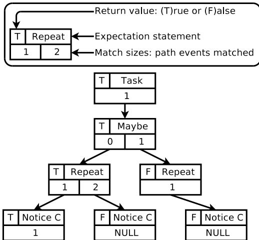
Figure 6: The search tree formed when matching the expectation and the path events in Figure 5.
