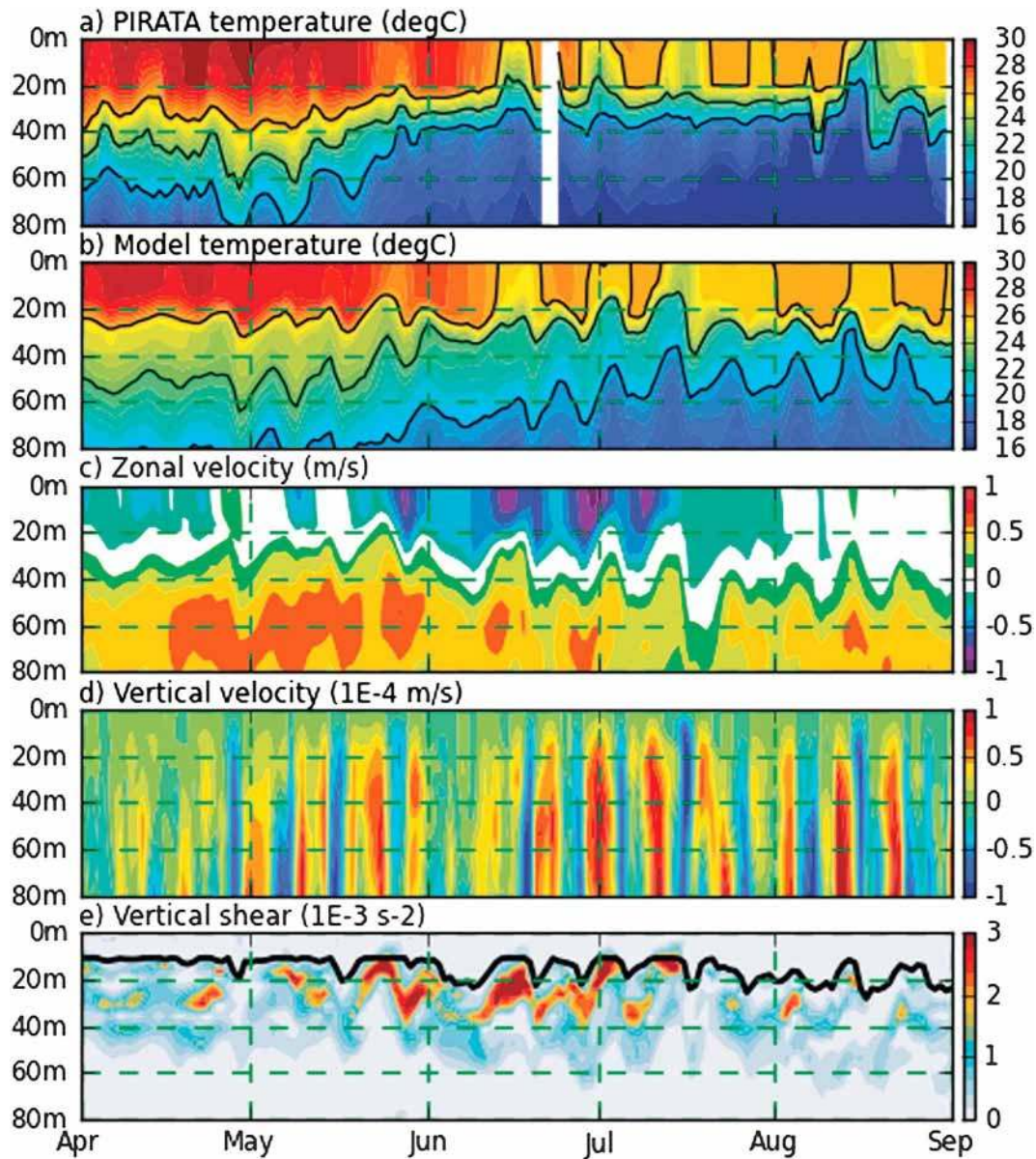
Figure 7. Time-depth diagrams at 0^\circ, 0^\circ of (a) observed Prediction and Research Moored Array in the Tropical Atlantic (PIRATA) temperature ( ^\circ\text{C} ), (b) model temperature ( ^\circ\text{C} ), (c) model zonal velocity ( \text{m/s} ), (d) model vertical velocity ( 10^{-4} \text{ m/s} ), and (e) vertical shear of horizontal velocities ( 10^{-3} \text{ s}^{-2} ). Black lines represent the 20^\circ , 23^\circ , and 26^\circ \text{C} isotherms in (a) and (b) and the depth of the model mixed layer in (e). Data are shown from April to August 2007. From Jouanno et al. (2013), their Figure 16 (reprinted by permission from American Meteorological Society).
