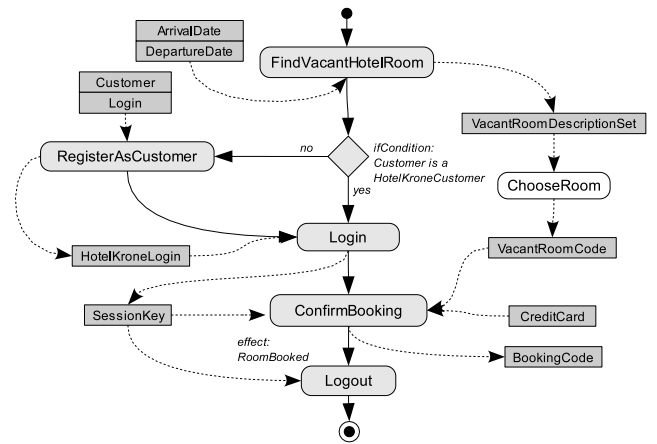
Figure 3: Booking agent process
