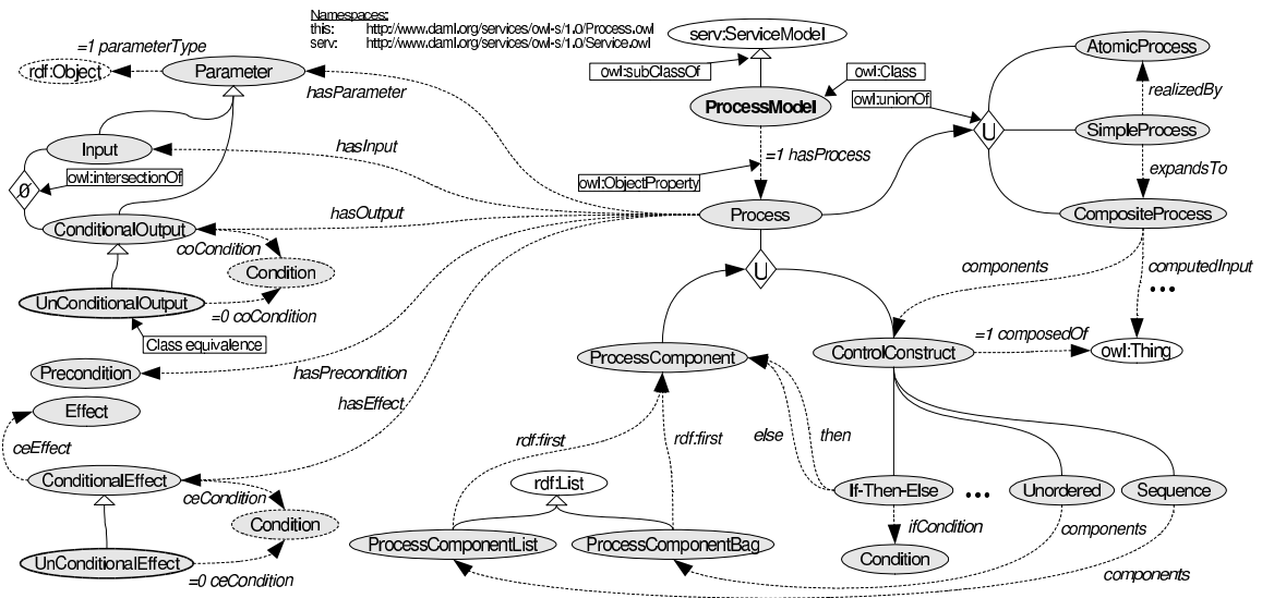
Figure 1: OWL-S process ontology
