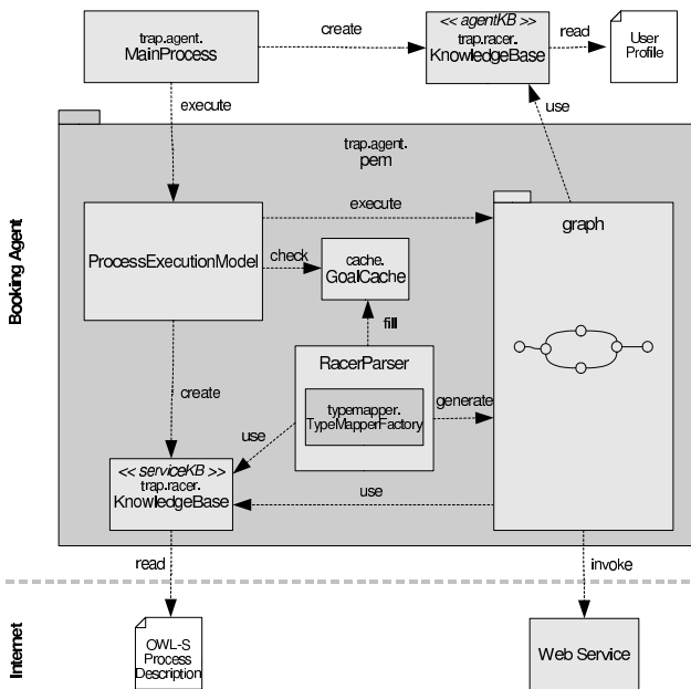
Figure 5: Execution model structure
