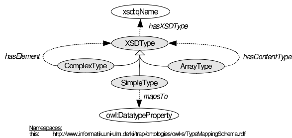
Figure 10: RDFS type mapping ontology
