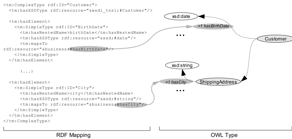
Figure 11: Example of an RDF-mapping
