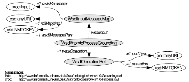
Figure 7: Modifications of the grounding ontology
