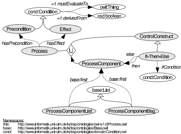
Figure 6: Modifications of the process ontology
