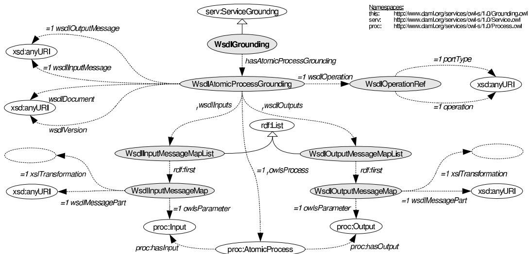
Figure 2: OWL-S grounding ontology
