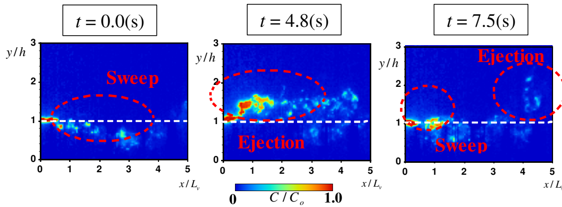
Fig.14 Simultaneous measurements of (a) instantaneous Reynolds stress by PIV and (c) instantaneous dye concentration by LIF in vegetated open-channel flow ( H = 15.0 cm, U_m = 12.0 cm/s, and vegetation density \lambda = 0.39 )
