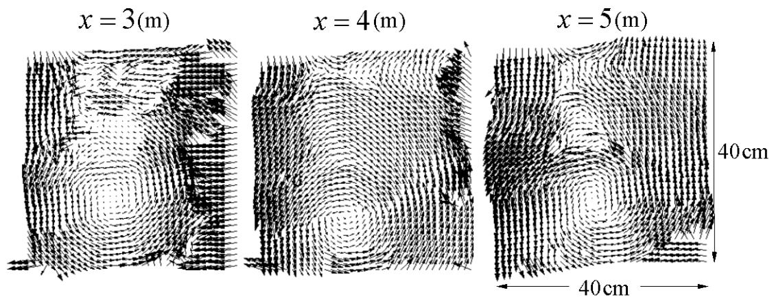
Fig.9 (a) Lagrangian PIV placed on auto-moving carrier, (b) Instantaneous velocity vectors on free-surface at every 1.0m in the streamwise direction ( H = 22.0 cm, D = 20.0 cm, B = 150 cm, B_f = 90 cm, and U_m = 15.0 cm/s)
