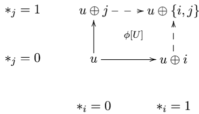
Fig. 3 2-up-uniformity: The orientations of the solid edges imply the orientations of the dashed edges . The top row contains vertices with j th entry equal to 1 and the bottom row vertices with j th entry equal to 0; the left column contains vertices with i th entry equal to 0, and the right column contains vertices with i th entry equal to 1
