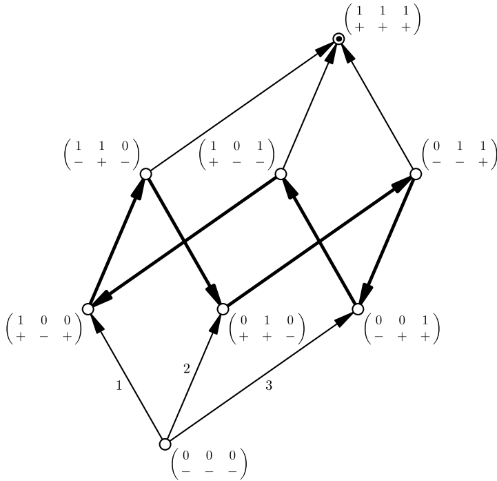
Fig. 1 A USO of the 3-cube; for each vertex, the orientation of incident edges is encoded with a sign vector in \{-, +\}^n ( - for an outgoing edge; + for an incoming edge). The unique global sink and a directed cycle are highlighted
