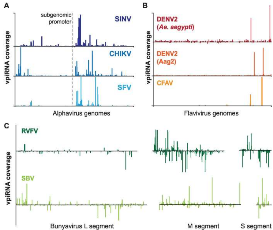
Fig 2. Viral piRNA profiles. piRNA distributions across the genomes of selected (A) alphaviruses, (B) flaviviruses, and (C) bunyaviruses. The plots depict published genome profiles of Sindbis virus (SINV) [29], chikungunya virus (CHIKV) [30], Semliki Forest virus (SFV) [31], dengue virus serotype 2 (DENV2) [35,36], cell fusing agent virus (CFAV) [34], Rift Valley fever virus (RVFV) [38], and Schmallenberg virus (SBV) [37]. For alphaviruses, the position of the subgenomic promoter is depicted. The piRNA coverage on the sense or antisense strand is shown as peaks above or below the x-axis, respectively. Please note that the plots are representations of piRNA profiles from multiple studies that used different ways of normalizing and presenting read counts. Therefore, the heights of the bars are arbitrary and do not allow a quantitative comparison between the different viruses.
