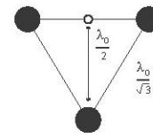
Figure 2. Inter-element distance of a hexagonal grid.
