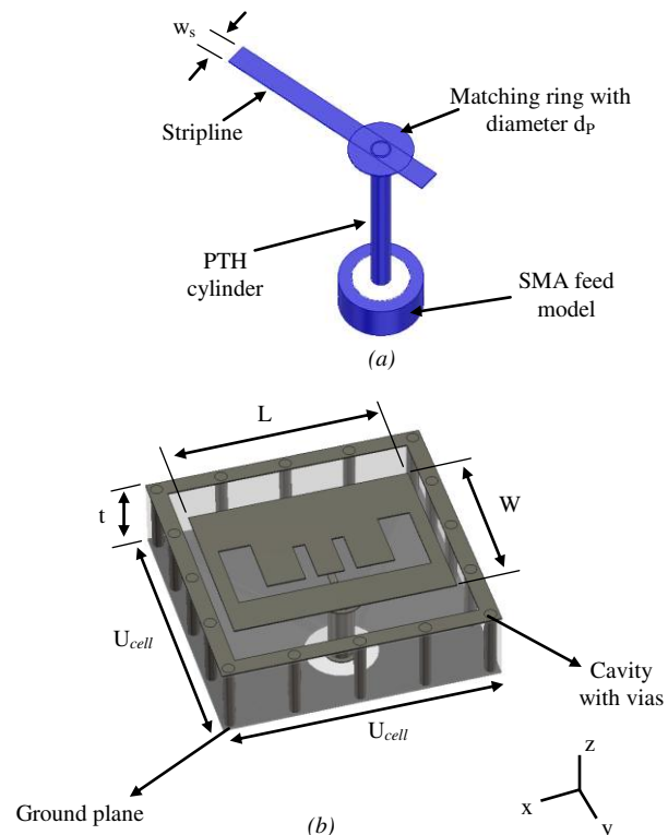
Fig. 3. Dual-band comb-slot-loaded antenna architecture. (a)- Feeding configuration and (b)- Unit-cell perspective view. Substrate maintained transparent for illustration.
