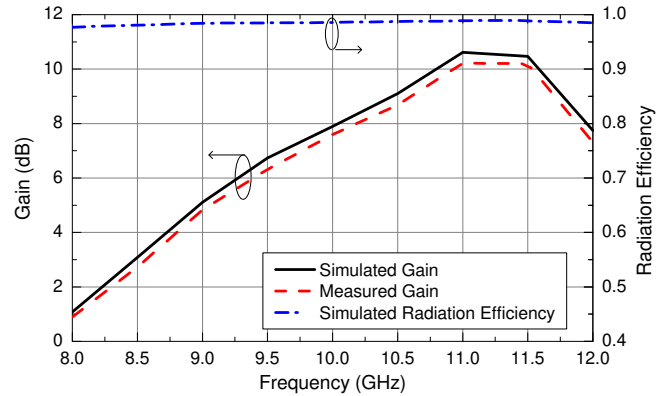
Fig. 18. Simulated and measured gain values and simulated radiation efficiency of the proposed antenna.
