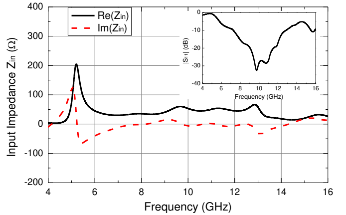
Fig. 5. Simulated input impedance and |S_{11}| of the proposed one-turn helical antenna.
