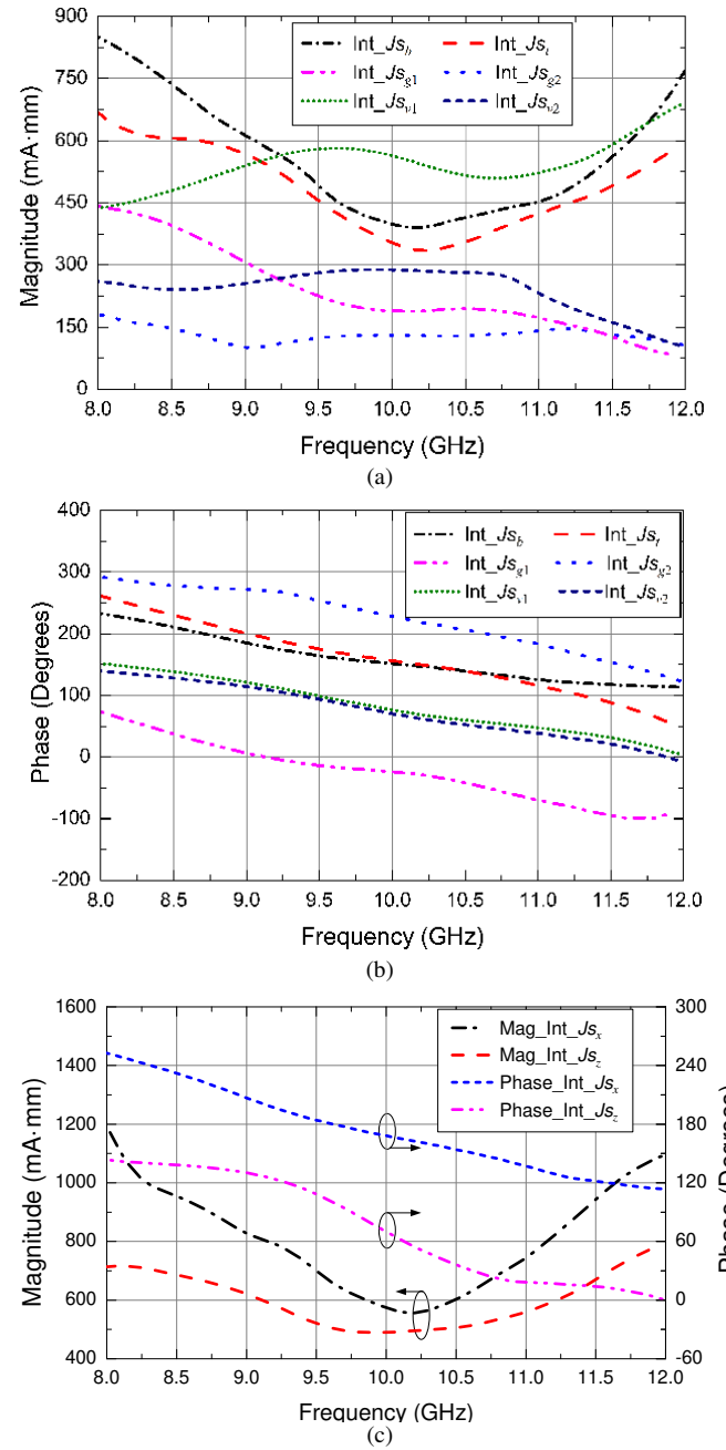
Fig. 3. (a) Magnitude and (b) phase values of surface current density integration of each segment on the helix and edge of the ground, (c) magnitude and phase values of combined total surface current density integrations of x and z directions.
