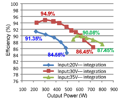
Fig. 17. The efficiency comparisons among the different input voltages at 400V output voltage and the three-voltage-level mode for the PIM converter.
