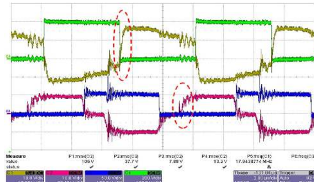
Fig. 14. ZVS waveforms in boost mode under three-voltage-level at 600W output power. CH1: V_{GS6} (10 V/div); CH2: V_{GS4} (10 V/div); CH3: V_{DS4} (50 V/div); CH4: V_{DS6} (200 V/div).
