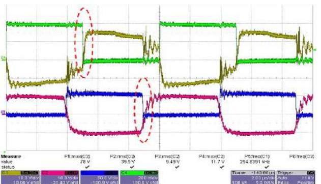
Fig. 11. ZVS waveforms in boost mode under two-voltage-level at 600W output power. CH1: V_{GS6} (10 V/div); CH2: V_{GS4} (10 V/div); CH3: V_{DS4} (50 V/div); CH4: V_{DS6} (200 V/div).
