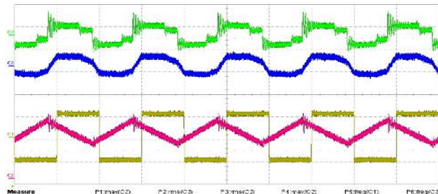
Fig. 13. Waveforms in boost mode under three-voltage-level at 600W output power. CH1: V_{CO} (200 V/div); CH2: i_{L1} (10 A/div); CH3: i_{L2} (10 A/div); CH4: V_{MO} (500 V/div).
