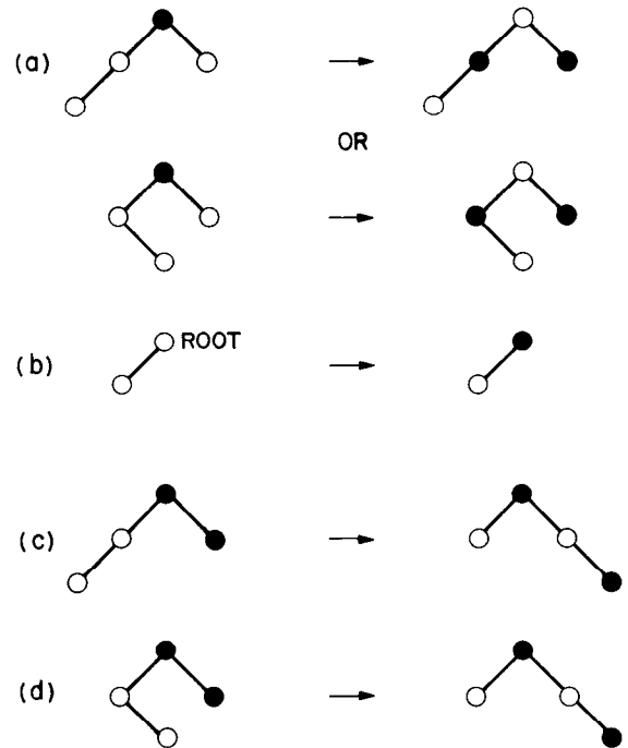
FIGURE 4. The Rebalancing Transformations in Red-Black Tree Insertion. Symmetric cases are omitted. Solid nodes are black; hollow nodes are red. All unshown children of red nodes are black. In cases (c) and (d) the bottommost black node can be missing.
