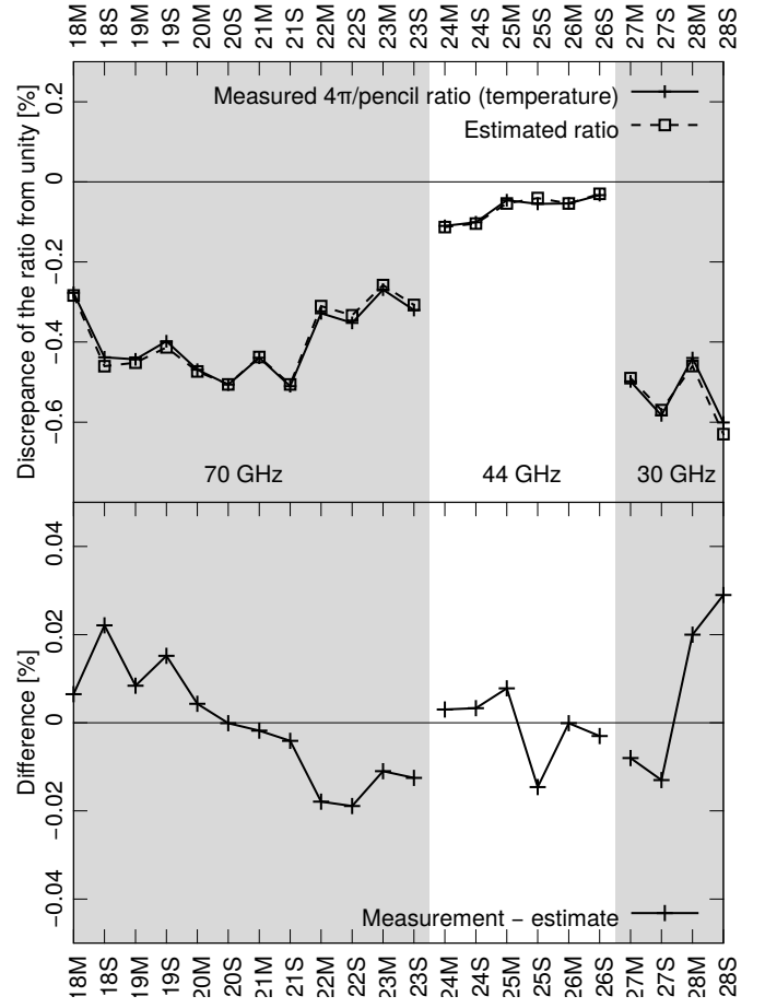
Fig. 8. Top: comparison between the measured and estimated ratios of the a_{\ell m} harmonic coefficients for the nominal maps (produced using the full knowledge of the beam B over the 4\pi sphere) and the maps produced under the assumption of a pencil beam. The estimate has been computed using Eq. (11). Bottom: difference between the measured ratio and the estimate. The agreement is better than 0.03 % for all 22 LFI radiometers.
