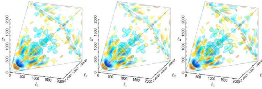
Fig. 6. Full 3D CMB bispectrum recovered from the Planck foreground-cleaned maps, including SMICA ( left ), NILC ( centre ) and SEVEM ( right ), using the hybrid Fourier mode coefficients illustrated in Fig. 9. These are plotted in three-dimensions with multipole coordinates \{\ell_1, \ell_2, \ell_3\} on the tetrahedral domain shown in Fig. 1 out to \ell_{\max} = 2000 . Several density contours are plotted with red positive and blue negative. The bispectra extracted from the different foreground-separated maps appear to be almost indistinguishable.
