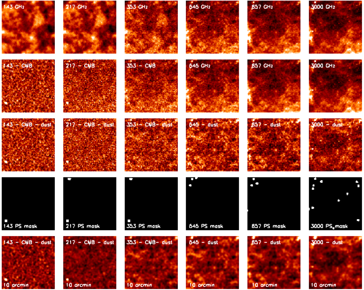
Fig. 4. Maps of the roughly 25 deg 2 of the SPC5 field, from left to right : 143, 217, 353, 545, 857, and 3000 GHz. From top to bottom : raw HFI and IRIS maps; CMB-cleaned maps; residual maps (CMB- and cirrus-cleaned); point source masks; and residual maps smoothed at 10' to highlight the CIB anisotropies. The joint structures clearly visible ( bottom row ) correspond to the anisotropies of the CIB.
