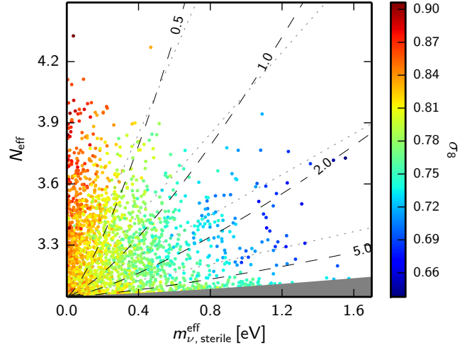
Fig. 32. Samples from Planck TT+lowP in the N_{\text{eff}}-m_{\nu, \text{sterile}}^{\text{eff}} plane, colour-coded by \sigma_8 , for models with one massive sterile neutrino family, with effective mass m_{\nu, \text{sterile}}^{\text{eff}} , and the three active neutrinos as in the base \Lambda CDM model. The physical mass of the sterile neutrino in the thermal scenario, m_{\nu, \text{sterile}}^{\text{thermal}} , is constant along the grey dashed lines, with the indicated mass in eV; the grey shading shows the region excluded by our prior m_{\nu, \text{sterile}}^{\text{thermal}} < 10 eV, which cuts out most of the area where the neutrinos behave nearly like dark matter. The physical mass in the Dodelson-Widrow scenario, m_{\nu, \text{sterile}}^{\text{DW}} , is constant along the dotted lines (with the value indicated on the adjacent dashed lines).
