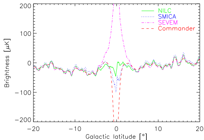
Fig. 26. Mean brightness vs. Galactic latitude, b , in the Planck CMB maps from Planck Collaboration IX (2016) , in the range |l| < 60^\circ . Solid green: N1LC; dotted blue: SMICA; dot-dashed magenta: SEVEM (all at 5 arcmin resolution); dashed red: baseline Commander model at 1^\circ resolution ( Planck Collaboration X 2016 ). The first three methods all use inpainting to fill masked regions around bright compact features in some or all of the input maps: pixels affected by this have been omitted from the averaging. High amplitudes close to b = 0 are due to residual foreground contamination.
