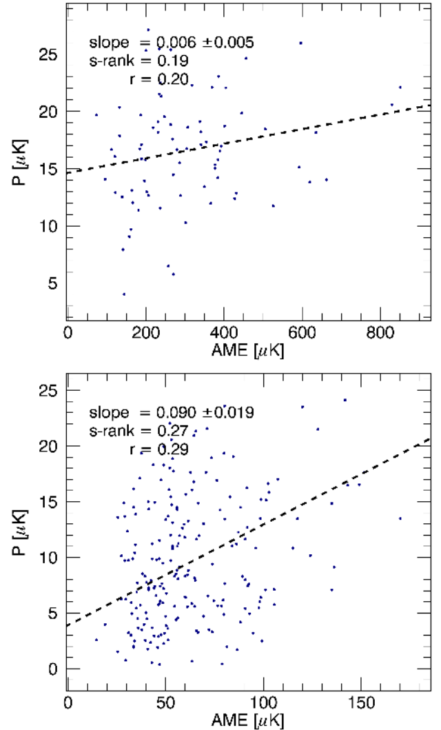
Fig. 34. T-T plots between the polarization and AME intensities (both in units of \mu\text{K} at 22.8 GHz). Top: Perseus; bottom: Pegasus plume. The scatter is mostly due to thermal noise in the polarization map (uncertainties in the polarization intensity in these regions are typically around 5\mu\text{K} ). The fitted slope gives the polarization fraction for the region, based on the linear fit (dashed line).
