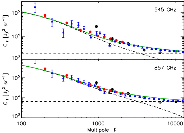
Fig. 17. Comparison of BLAST and HFI measurements at 545 and 857 GHz. HFI data points are the red circles; BLAST data points are the black diamonds. They were colour-corrected for the comparison (the colour was computed using the CIB SED of Gispert et al. (2000) , integrated through the BLAST and HFI bandpass filters). The dashed line is the BLAST shot noise (also colour-corrected). Also shown is the BLAST best-fit clustering model (black dash-dotted line) and the total contribution (shot noise plus clustering; continuous green line). It provides a good fit to the Planck data. Finally, we report in this figure a revised version of the SPIRE data points from Amblard et al. (2011) (blue triangles from Fig. 18, see text for more details).
