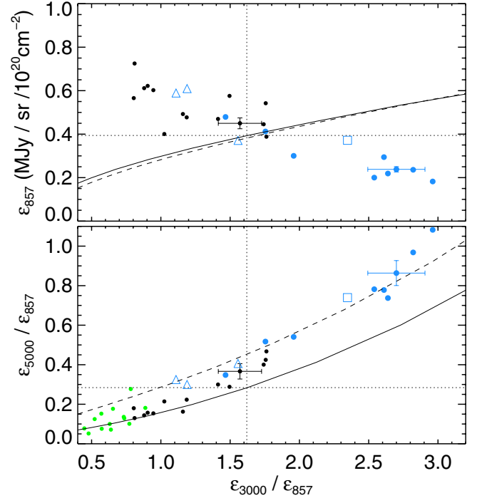
Fig. 22. Top: dust emission per \text{N}_{\text{HI}} at 857 GHz versus the 3000/857 GHz (100/350 \mu\text{m} ) ratio. Local (black), IVC (blue – dot is IV Arch, triangle IV/LLIV Arch, square Complex K), residual (green). Solid line is the DustEM model for the diffuse ISM (Compiègne et al. 2011), with radiation field variations from G = 0.1 to G = 5 . Dashed line is the same model but with a relative abundance of VSGs four times higher than the standard diffuse ISM value. Dotted lines gives the local ISM fiducial values ( G = 1.0 ). Typical uncertainties are shown for each H I component. Bottom: 5000/857 GHz (60/350 \mu\text{m} ) ratio as a function of the 3000/857 GHz (100/350 \mu\text{m} ) ratio.
