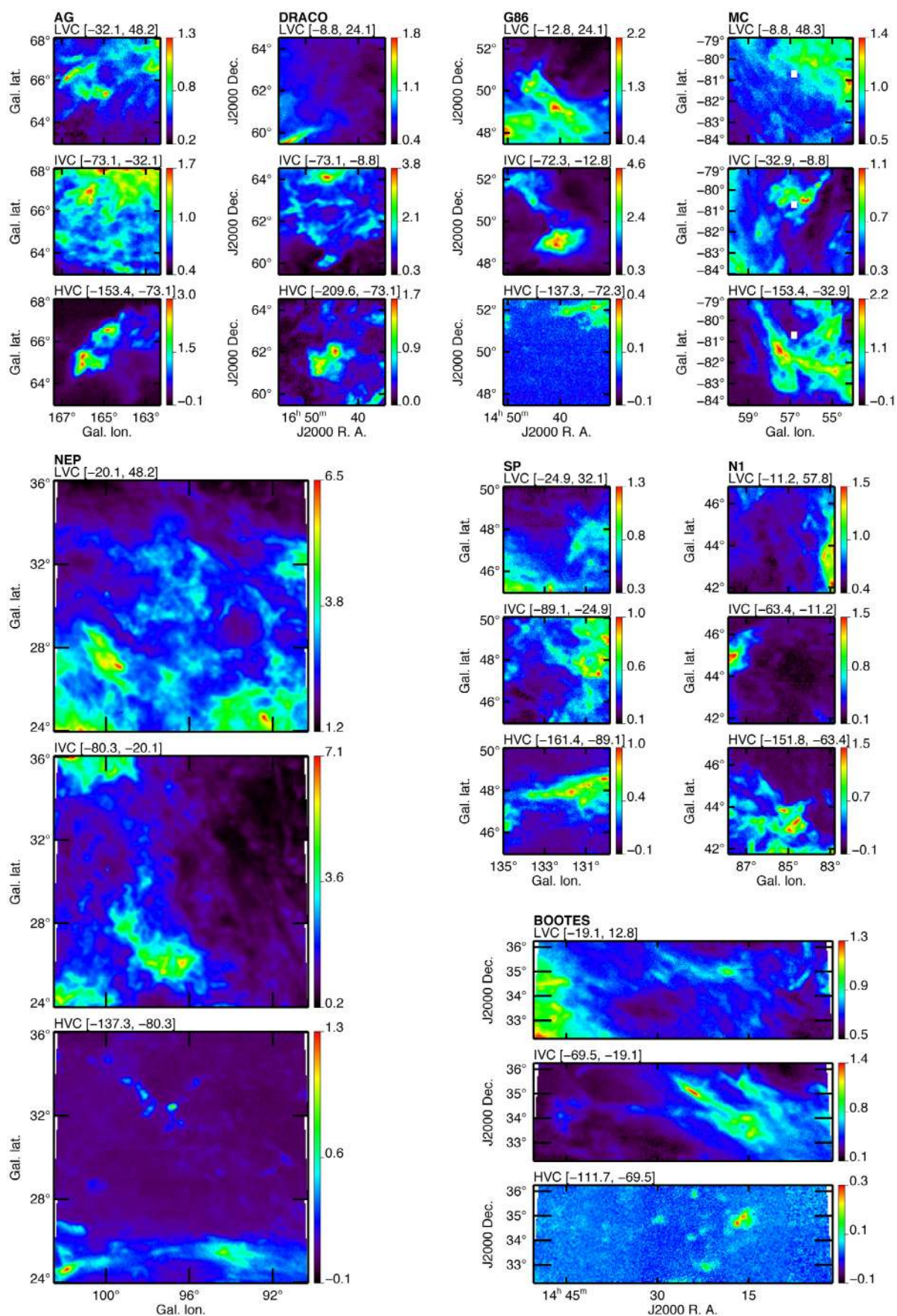
Fig. 2. H I column density maps in units of 10^{20} \text{ cm}^{-2} for the AG, DRACO, G86, MC, NEP, SP, N1 and BOOTES fields. To show the full detail, the range is different for each H I component for a given field. The LSR velocity range used to compute each H I component map is given in brackets (unit is \text{km s}^{-1} ).
