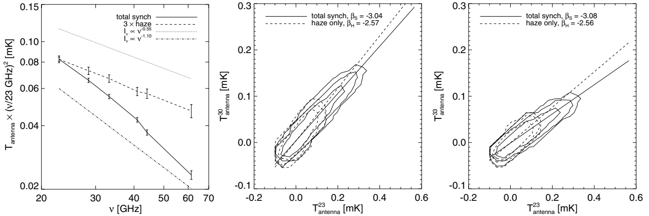
Fig. 8. Left: spectrum measured from the residual in Fig. 6 in the region |\ell| < 35^\circ , -35^\circ < b < -10^\circ . The haze spectrum is very nearly a power law with spectral index \beta_H = -2.56 , while the total synchrotron emission in the region has a spectral index of \beta_S = -3.1 (see Sect. 4.3), significantly softer than the haze emission. This spectrum should be free from biases caused by template uncertainties. Middle and right: scatter plots (shown in contours) for both the haze (dotted) and total synchrotron (solid) emission using WMAP 23–33 GHz and Planck 30 GHz.
