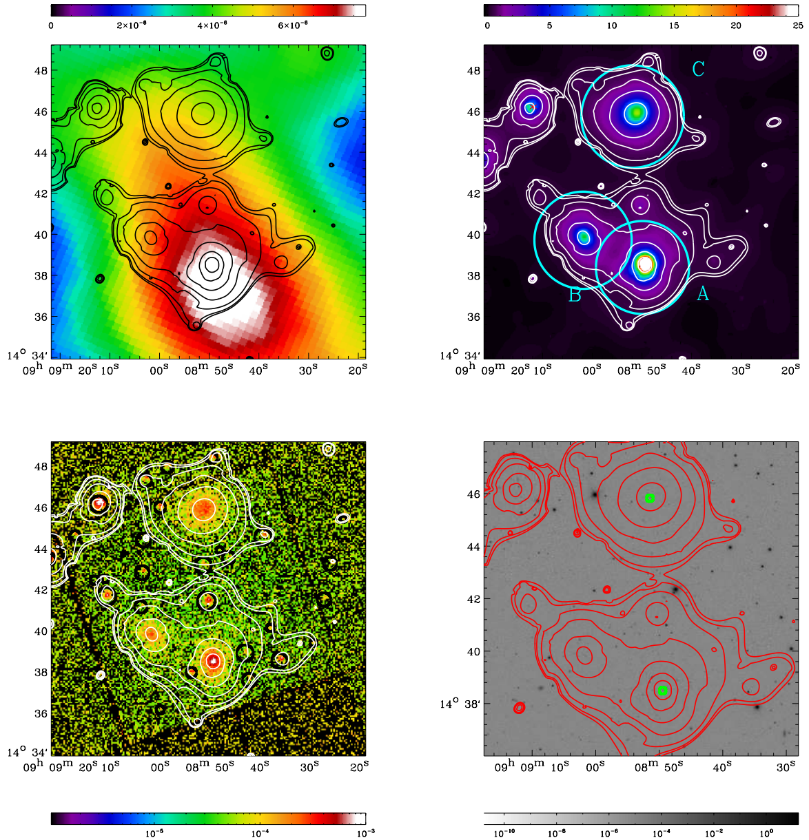
Fig. 1. Triple systems PLCKG214.6+37.0. Left upper panel: Planck SZ reconstructed map (derived from the Modified Internal Linear Combination Analysis, Hurier et al. 2010), oversampled and smoothed for display purposes. Right upper panel: XMM-Newton wavelet filtered image in the [0.5–2.5] keV range (Sect. 2.2). The three components of PLCKG214.6+37.0 are marked with circles (with radius R_{500} , see Table 1) and indicated with letters as in the text. The X-ray structure visible in the north-east (marked with an asterisk) is likely associated with the active galaxy SDSSJ090912.15 + 144613.7, with a spectroscopic redshift z = 0.767 . Left lower panel: Raw MOS count rate (counts s^{-1} ) image in the [0.5–2.5] keV range, corrected for vignetting. The black circles mark the point sources detected by our algorithm, which we masked during the analysis (Sect. 2.2). The pixel size in this image is 4.35'' . Right lower panel: SDSS r -band image of the PLCKG214.6+37.0 field. In all panels, north is up and east to the left, and we overlay X-ray contours, computed on the wavelet-filtered image logarithmically spaced starting from the level where a connection is seen between all components (Sect. 3.4).
