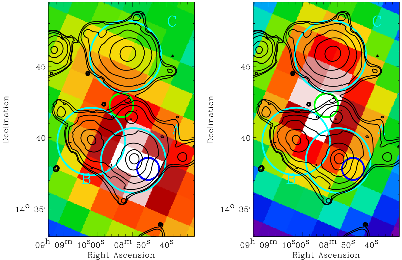
Fig. 8. MILCA y -map ( left panel ) compared with the pseudo pressure X-ray map degraded to the y -map resolution ( right panel ). X-ray contours and cyan circles indicating the three components are over-plotted to guide the eye. The green and blue circles mark the positions of the peaks in the y -map and in the pseudo-pressure distribution, respectively.
