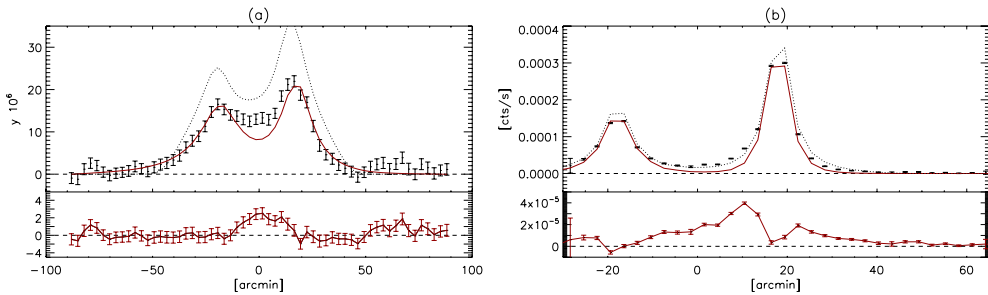
Fig. 6. 1D a) tSZ and b) X-ray profiles and residuals for the best-fit models of the A399 and A401 clusters. The red curve corresponds to the GNF2 model. The dotted lines are the model from Sakelliou & Ponman (2004).
