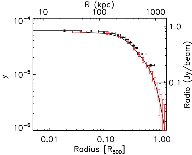
Fig. 10: Comparison of the \gamma (black) and diffuse radio (red) global radio profiles in Coma. The radio profile has been convolved to 10 arcmin resolution to match the Planck FWHM and simply rescaled by the multiplication factor derived from the linear regression shown in Fig. 9. The radio errors are dominated by uncertainties in the zero level due to a weak bowling effect resulting from the lack of short interferometer spacings.
