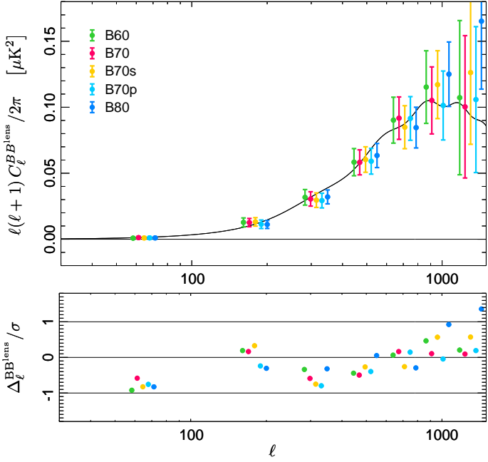
Figure 7. Cross-correlation of our B -mode template with the SMICA polarization map using masks of different levels of conservatism. The data points show the lensing C_\ell^{BB} band-powers estimated using masks that preserve a sky fraction of about 60% (labelled B60), 70% ('B70'), and 80% ('B80'), and that are targeted to the foreground emission in temperature (see Sect. 7.2.1); as well as using the 68% 'B70s' mask, which allows for a more conservative masking of the extragalactic objects (see Sect. 7.2.2), and the 68% polarization-targeted 'B70p' mask (see Sect. 7.2.3). The residuals with respect to the model in units of the 1\sigma band-power uncertainties are shown in the lower panel. The good agreement of all cases within error-bars provides a robustness test against foregrounds, as discussed in Sect. 7.2.
