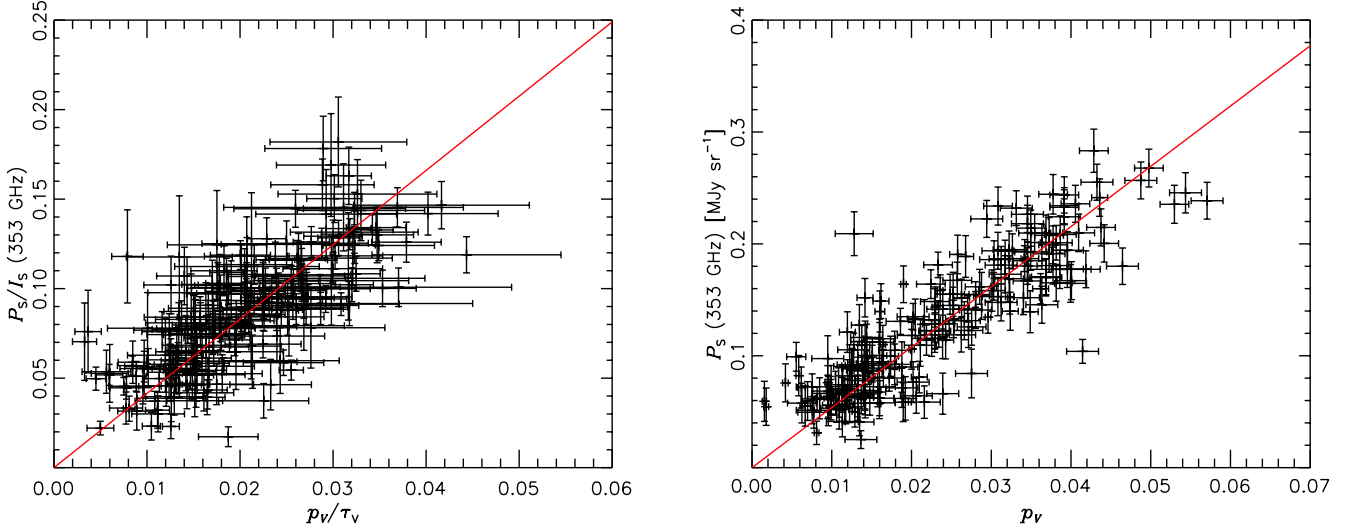
Fig. C.3. Left: Correlation of debiased polarization fraction in emission with that in extinction (Pearson coefficient 0.74). Right: Correlation of the debiased polarized emission (in MJy sr -1 ) with starlight polarization degree (Pearson coefficient 0.87). The range corresponds to one quadrant in Fig. 7. The fits are forced to go through the origin and have slopes R_{S/V} = 4.18 \pm 0.04 ( \chi_r^2 = 1.77 ) and R_{P/p} = (5.41 \pm 0.04) MJy sr -1 ( \chi_r^2 = 2.98 ), respectively.
