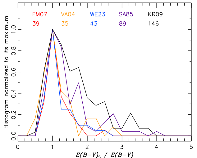
Fig. 2. Normalized histograms of the column density ratio R_{\tau_S} for those lines of sight passing the first two selection criteria for S/N and diffuse ISM, for the independent FM07 (red), VA04 (orange), WE23 (blue), SA85 (mauve), and KR09 (black) samples. The number of stars in each sample is indicated.
