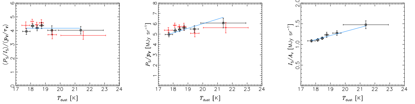
Fig. C.2. Left: Mean R_{S/V} as a function of the mean T_{\text{dust}} , each plotted with the standard deviation, in bins of equal number. Two versions of the Planck data have been used: with (black) and without (red) correction for leakage of intensity into polarization. Middle: The same, but for R_{P/p} . Right: The same, but for I_S/A_V . The blue curves, motivated in the right panel, show the expected response of the ratios to an increase in T_{\text{dust}} , according to a simple model in which the subset of grains that are polarizing had the same temperature as characterized the total emission (see text).
