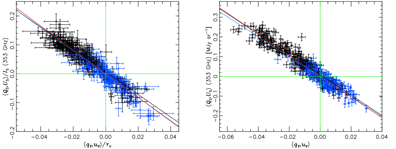
Fig. 7. Left : Correlation of polarization fractions in emission with those in extinction for the joint fit in Q (black) and U (blue). Using Eq. 15 the best linear fit (red line) has slope and y -intercept -4.13 \pm 0.06 and 0.0006 \pm 0.0007 , respectively. The Pearson correlation coefficient is -0.93 and \chi_r^2 = 1.64 . Right : Correlation of polarized intensity in emission ( \text{MJy sr}^{-1} ) with the degree of interstellar polarization. Using Eq. 16, the best linear fit (red line) has slope and y -intercept (-5.32 \pm 0.06) \text{ MJy sr}^{-1} and (0.0020 \pm 0.0009) \text{ MJy sr}^{-1} , respectively. The Pearson correlation coefficient is -0.95 and \chi_r^2 = 2.29 . Lines for the independent fits to Q (black) and U (blue) are also shown.
