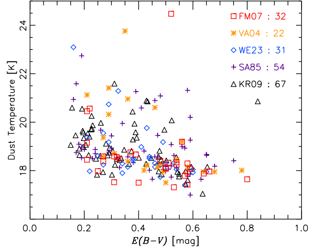
Fig. C.1. Planck line of sight dust temperature T_{\text{dust}} (Planck Collaboration XI 2014) and the column density to the star, E(B - V) , for the independent samples.
