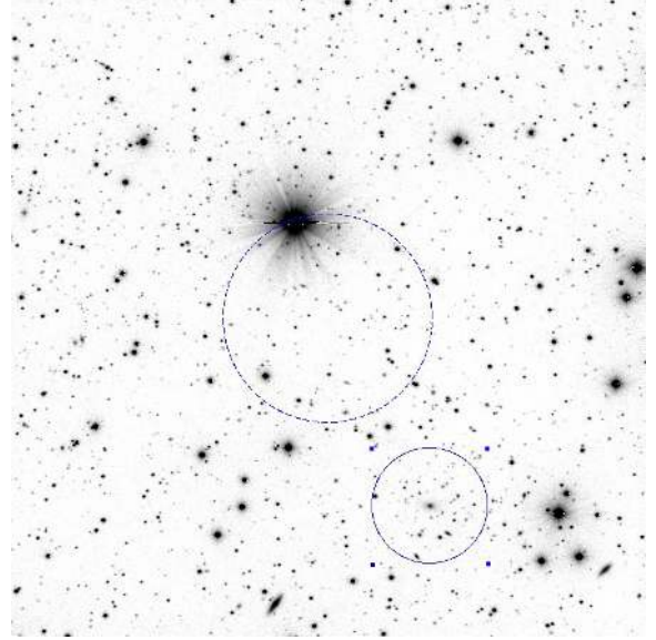
Fig. 11. PSZ1 G066.01-23.30 RTT150 r' -band image centred on the Planck SZ source coordinates, dashed 2' radius circle shows approximate Planck SZ source coordinates uncertainty. The position of the optical galaxy cluster is shown with a solid circle.
