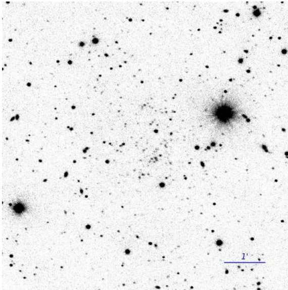
Fig. 10. PSZ1 G084.04+58.75 RTT150 r' -band image. This cluster is too distant to be identified with SDSS ( z = 0.731 ).
