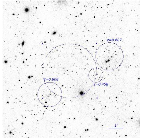
Fig. 12. PSZ1 G070.91+49.26 RTT150 r' -band image centred on the Planck SZ source coordinates, dashed 2' radius circle shows approximate Planck SZ source coordinates uncertainty. In addition to a double cluster at z \approx 0.61 , there is a smaller foreground cluster at z \approx 0.46 (shown with solid circles).
