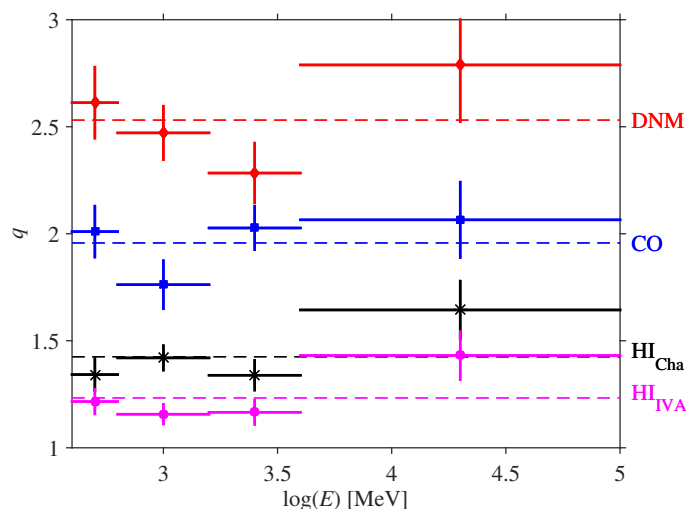
Fig. 6. Spectral variation, relative to the local interstellar spectrum q_{LIS} , of the \gamma -ray emissivities obtained for the local gas components in the \gamma+A_{VQ} analysis. The q_{CO} value is given in units of 10^{20} \text{ cm}^{-2} \text{ K}^{-1} \text{ km}^{-1} \text{ s} , q_{DNM} in 8 \times 10^{20} \text{ cm}^{-2} \text{ mag}^{-1} , and the H I emissivities refer to the optically thin H I case. The dotted lines mark the mean emissivities.
