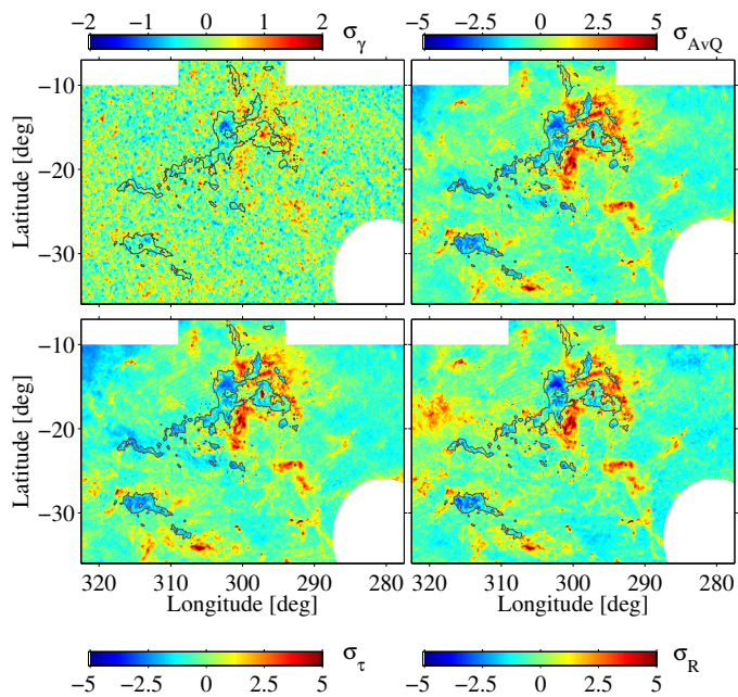
Fig. D.1. Maps of residuals (data minus best-fit model, in sigma units) obtained when fitting the \gamma -ray, A_{\text{VQ}} , R , or \tau_{353} data (clockwise) with optically thin H I and W_{\text{CO}} , but no DNM. In all plots, the grey contours outline the shape of the CO clouds at the 2.3 \text{ K km s}^{-1} level.
