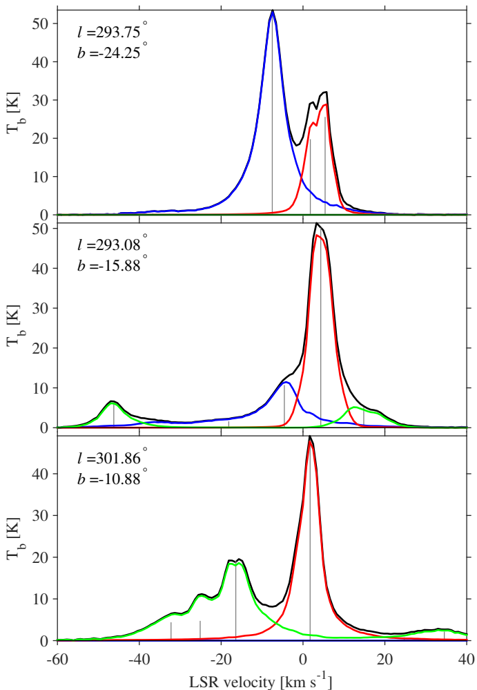
Fig. A.2. H I GASS spectra, in brightness temperature, measured toward the three directions indicated on the plots. The best line fits attributed to the local (red), IVA (blue), and Galactic (green) components sum up as the black curve, which closely follows the original data. The grey lines indicate the central velocity and temperature of the individual lines that contribute to a component.
