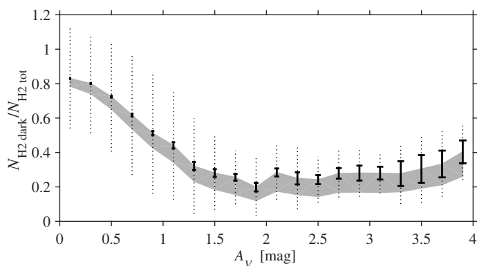
Fig. 17. Evolution of the CO-dark to total H 2 column-density ratio with the 2MASS visual extinction. The molecular fraction in the DNM varies from 50 % (lower grey bound) to 100 % (upper bound). The gas column densities in the CO and DNM phases have been obtained with the X_{\text{CO}\gamma} factor and the \gamma -ray N_{\text{HDNM}} map from the \gamma+A_{VQ} analysis. The other analyses yield equivalent curves. The thick and dotted lines respectively give the standard error of the mean and the standard deviation of the ratios for each A_V bin, in the case of a fully molecular DNM.
