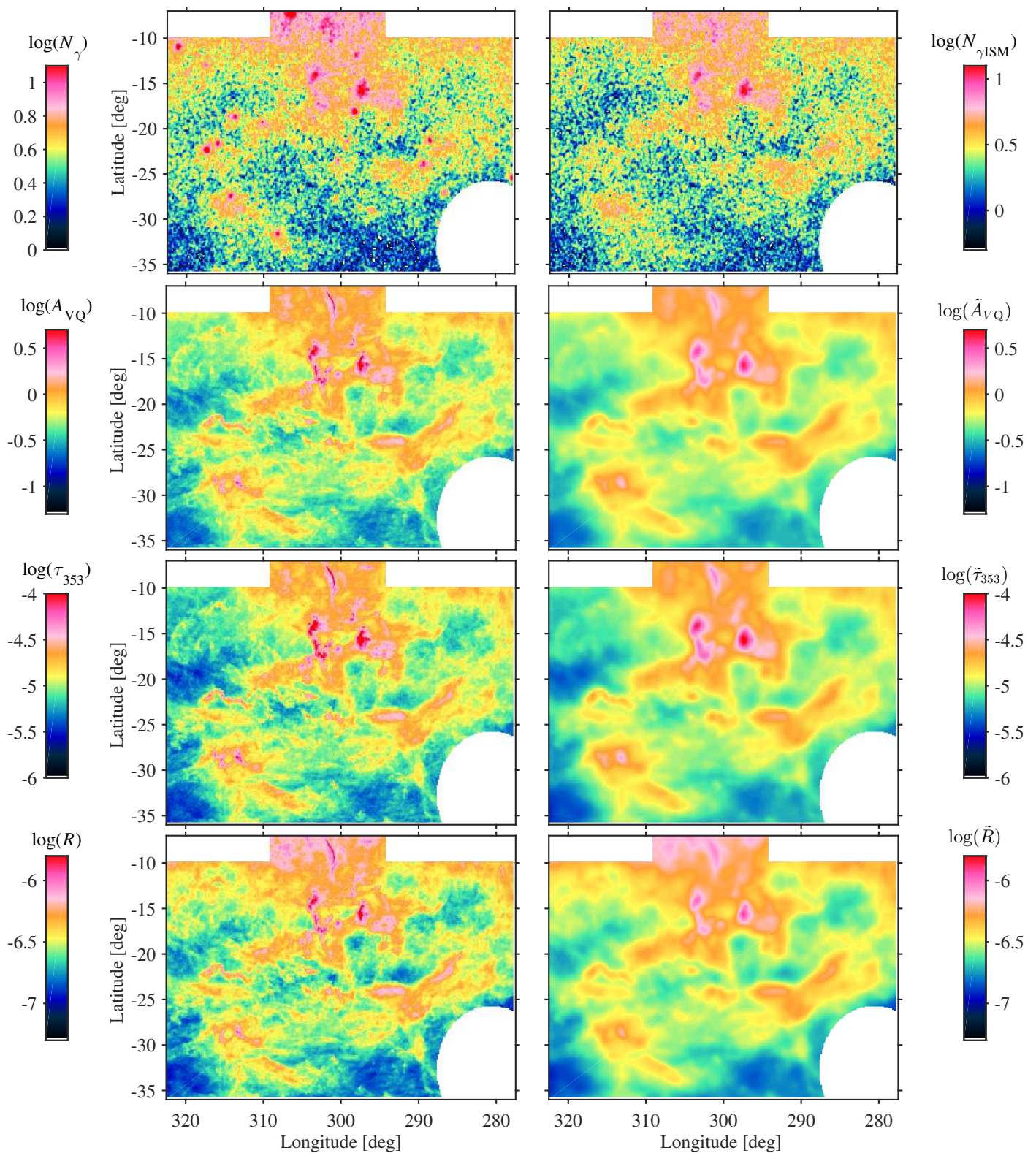
Fig. 1. Maps toward the Chamaeleon region of the \gamma -ray counts recorded in the 0.4 – 100 GeV band and of the dust quantities (modified extinction A_{VQ} in magnitudes, optical depth \tau_{353} , and radiance R in \text{W m}^{-2} \text{sr}^{-1} ). The total \gamma -ray photon counts are shown on the left and those spawned by cosmic-ray interactions with gas (after subtraction of other ancillary components) on the right. The \gamma -ray maps have been constructed on a 7:5 pixel grid and smoothed with a Gaussian kernel of 0:1 for display. The dust quantities are shown at 5' resolution in the left panels, and at the Fermi LAT resolution on the right (after convolution with the energy-dependent response function of the LAT, assuming the local interstellar \gamma -ray spectrum over the 0.4–100 GeV band, tilded variables). Regions excluded from the analysis have been masked out.
