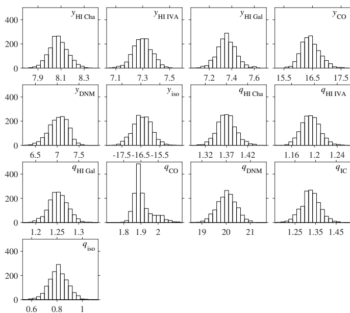
Fig. 4. Number distributions of the model coefficients obtained in the 1500 jackknife fits of the \gamma+A_{VQ} analysis for the optically thin H I case and overall energy band in \gamma rays. The y_{\text{HI},i} and y_{\text{DNM}} quantities are in units of 10^{-22} mag cm ^2 , y_{\text{CO}} in 10^{-2} mag K ^{-1} km ^{-1} s, y_{\text{iso}} in 10^{-2} mag, q_{\text{CO}} in 10^{20} cm ^{-2} K ^{-1} km ^{-1} s, and q_{\text{DNM}} in 10^{20} cm ^{-2} mag ^{-1} . The q_{\text{HI},i} , q_{\text{IC}} , and q_{\text{iso}} values are simple normalization factors.
