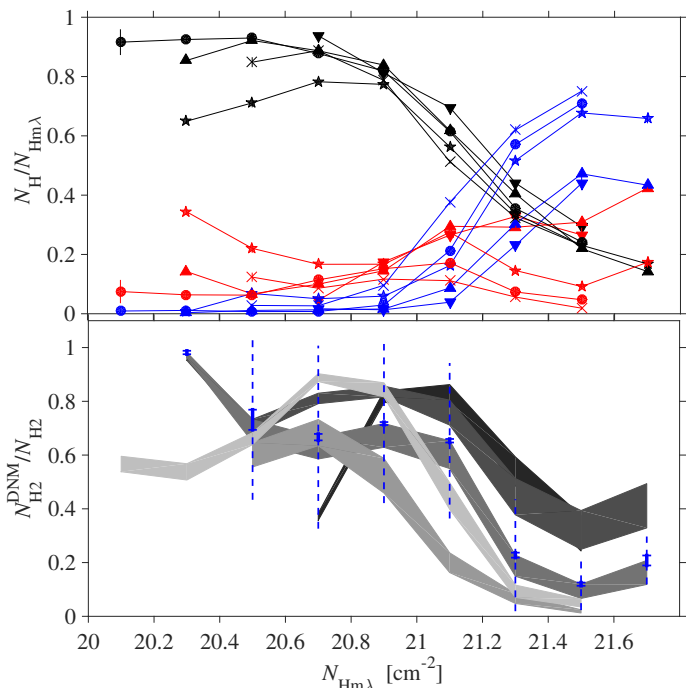
Fig. 16. Variations with N_{\text{Hm}\lambda} , in five separate clouds, of the fraction of the total column density in each phase ( upper panel , H I in black, DNM in red, CO in blue) and of the fraction of the total \text{H}_2 column density that is CO dark ( lower panel ). Downward and upward triangles, stars, crosses, and circles refer to Musca, Cham I, Cham II+III, Cham East I, and Cham East II, respectively. The dark to light grey curves correspond to the clouds in the same order. The shaded areas cover the chosen uncertainty in DNM composition from 50% to 100% \text{H}_2 . The dotted and solid error bars give the standard deviations and errors on the mean in each N_{\text{H}} bin; they are shown for only one cloud and the fully molecular DNM case.
