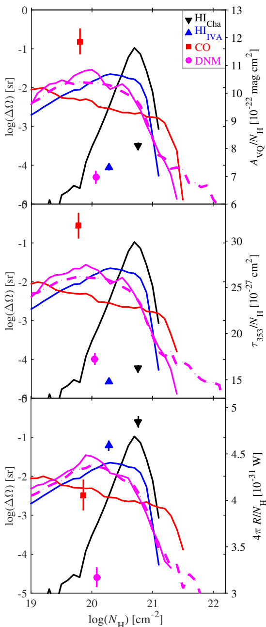
Fig. 14. Solid angle distributions of N_{\text{H}} in the different gas phases from the three analyses: in the optically thin H I gas of the local cloud and intermediate-velocity arc; in the DNM gas as traced in \gamma rays ( solid ) or in dust ( dashed ); and in the CO phase with the \gamma -ray derived X_{\text{CO}} factors. The data points give the mean dust properties ( A_{\text{VQ}}/N_{\text{H}} , opacity, and specific power) in each phase. They are placed at the position of the average column density in each phase. The insert gives the colour code and symbol for each phase.
