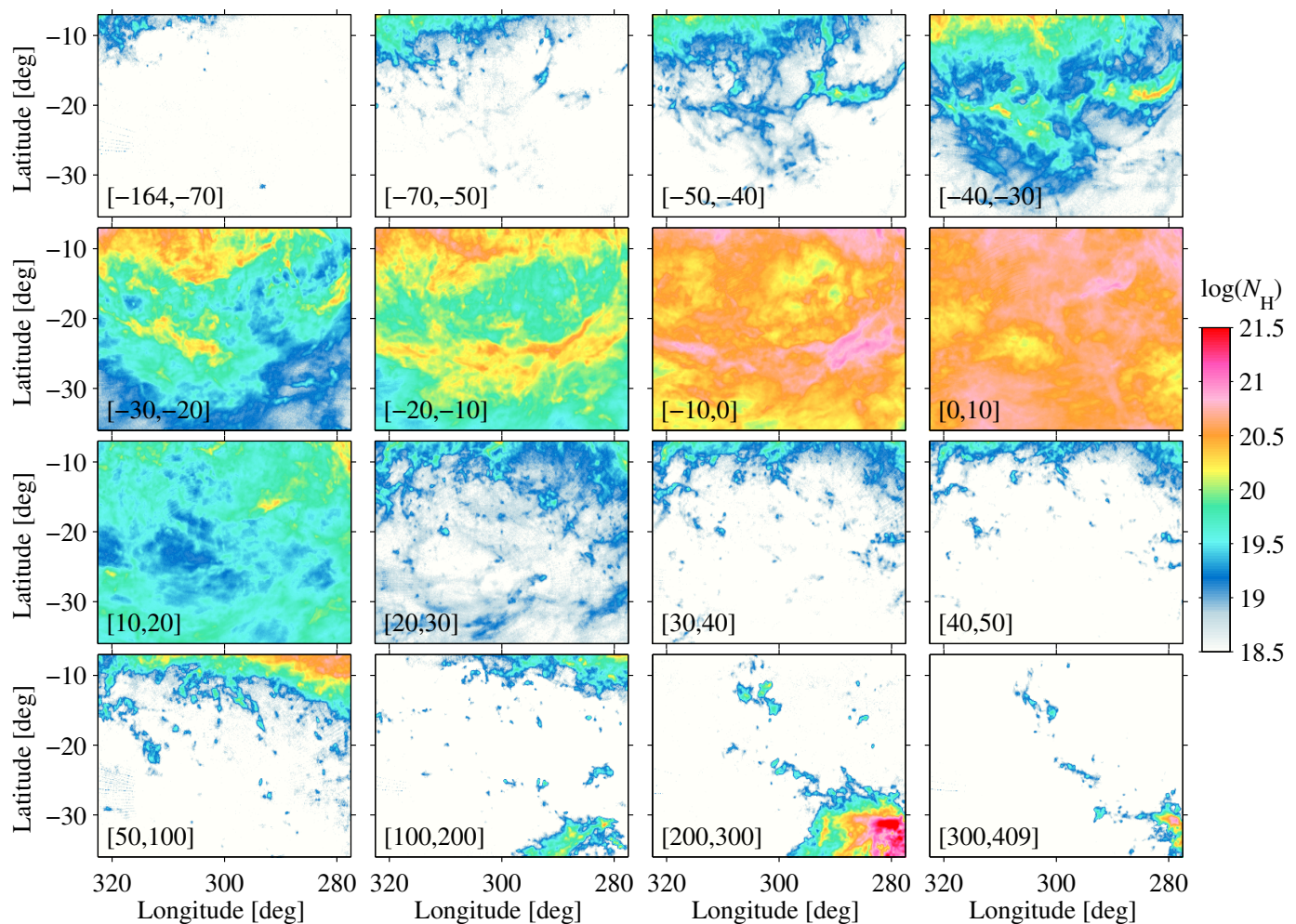
Fig. A.1. Maps of the N_{\text{H I}} column densities (in \text{cm}^{-2} ) obtained at 14.5 resolution from the GASS survey for optically thin emission and integrated over contiguous velocity intervals between the values given in \text{km s}^{-1} on the lower left corner of each map.
