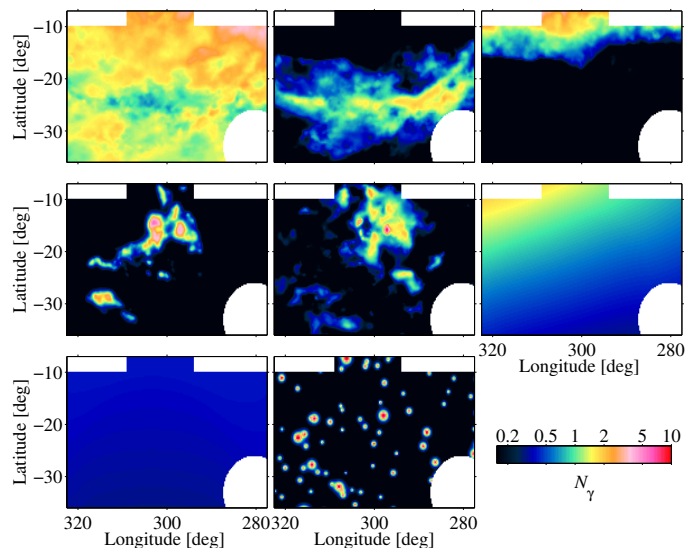
Fig. 3. Photon yields, on a 0.125 -pixel grid, from the various components of the \gamma -ray model in the 0.4 – 100 GeV band. From left to right and from top to bottom, the yields come from the N_{\text{H I}} column densities in the local, IVA, and Galactic disc clouds, the W_{\text{CO}} intensity in the local clouds, the N_{\text{H DNM}} column density derived from A_{\text{VQ}} , the IC emission, the isotropic background, and point sources.
