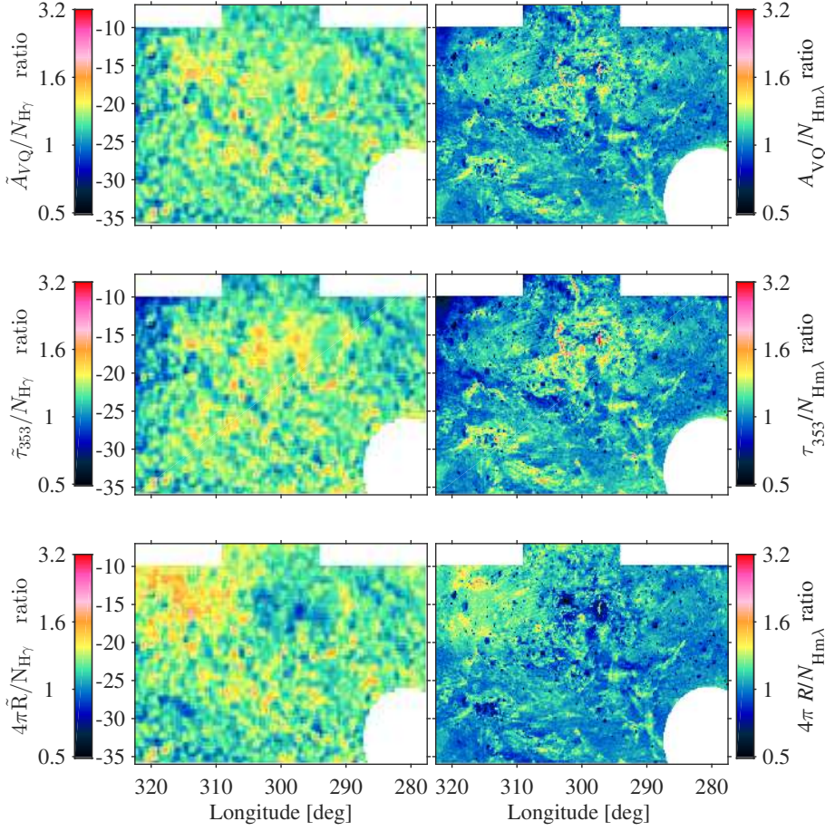
Fig. 12. Spatial variations of the dust properties per gas nucleon, relative to the average values obtained at low N_{\text{H}} , in the (1 - 2.2) \times 10^{21} \text{ cm}^{-2} interval for N_{\text{H}\gamma} (left column), and in the (0.4 - 2) \times 10^{21} \text{ cm}^{-2} interval for N_{\text{Hm}\lambda} (right column). As in the previous figure, the total gas is measured by N_{\text{H}\gamma} on a 0.375 pixel grid (left) and by N_{\text{Hm}\lambda} on a 0.125 pixel grid (right). Colours saturate for ratios below 0.5 and above 3.2 .
