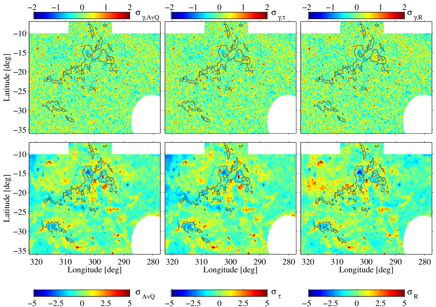
Fig. 5. Upper row: photon count residuals between the data and best-fit model, in sigma units on a 0^\circ 125 -pixel grid, in the 0.4–100 GeV band, with the DNM template from the dust A_{VQ} (left), \tau_{353} (middle), or radiance (right). Lower row: dust residuals between the data and best-fit model, in sigma units, for the fit in A_{VQ} (left), \tau_{353} (middle), and radiance (right). The grey contours outline the CO clouds at the 2.3 \text{ K km s}^{-1} level.
