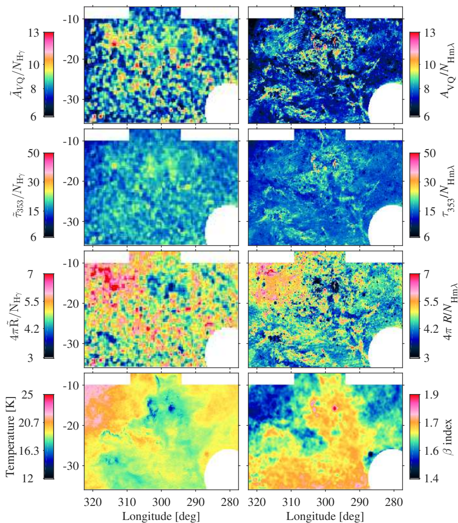
Fig. 11. Three upper rows: spatial variations of the dust properties per gas nucleon with the total gas measured by N_{H\gamma} on a 0^\circ:375 pixel grid (left) and by N_{Hm\lambda} on a 0^\circ:125 pixel grid (right). Lower row: colour temperature and \beta index of the dust SED, measured at 5' resolution by Planck Collaboration XI (2014) and displayed on a 0^\circ:125 pixel grid. The A_{VQ}/N_H values are in units of 10^{-22} mag \text{cm}^2 , \tau_{353}/N_H in 10^{-27} \text{cm}^2 , and 4\pi R/N_H in 10^{-31} W.
