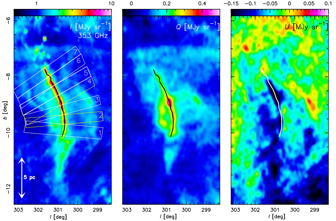
Fig. 1. Planck 353 GHz Stokes parameter maps of Musca (in \text{MJy sr}^{-1} ). The total intensity map is at a resolution of 4'8 , while the Q and U maps are smoothed to a resolution of 9'6 for better visualization. The crest of the filament traced on the I map is drawn in black (on the I and Q maps) and white (on the U map). The boxes drawn on the I map, numbered from 1 to 7, show the regions from which the mean profiles are derived (see Fig. 2).
