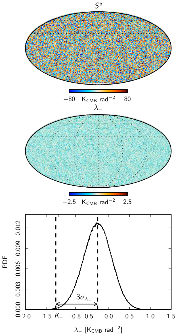
Fig. A.1. Filtered realization of the Gaussian dust sky ( upper panel ) and the corresponding eigenvalue \lambda_- ( middle panel ). The distribution of the eigenvalue \lambda_- ( lower panel ) over the unmasked pixels is Gaussian.
