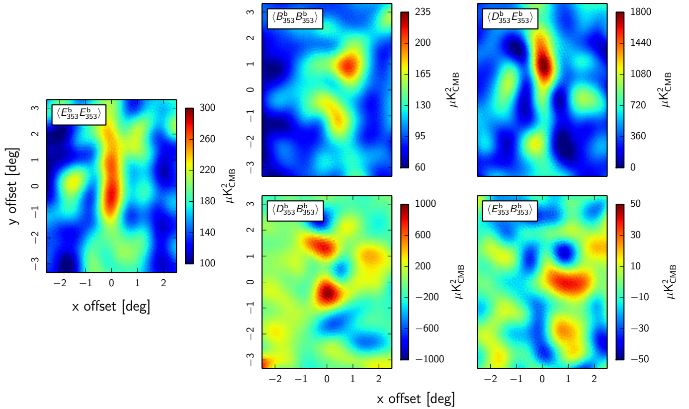
Fig. 11. Mean images of the Planck \langle E_{353}^b E_{353}^b \rangle , \langle B_{353}^b B_{353}^b \rangle , \langle D_{353}^b D_{353}^b \rangle , \langle D_{353}^b B_{353}^b \rangle , and \langle E_{353}^b B_{353}^b \rangle maps over the \lambda_- filaments.
