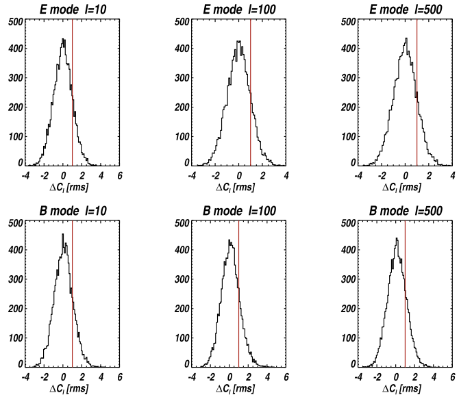
Fig. 4. Distribution of \Delta C_\ell^{EE} (top) and \Delta C_\ell^{BB} (bottom) for \sigma_\epsilon = 1\% polar efficiency errors for multipoles \ell = 10 , \ell = 100 , \ell = 500 , normalized to their rms (red line).
