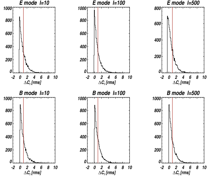
Fig. 3. Distribution of \Delta C_\ell^{EE} (top) and \Delta C_\ell^{BB} (bottom) for \sigma_\gamma = 0.2\% gain errors for multipoles \ell = 10 , \ell = 100 , \ell = 500 , normalized to their rms (red line).
