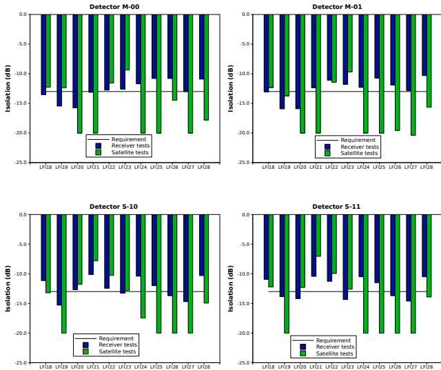
Fig. 13. Summary of isolation measured at receiver and satellite levels.
