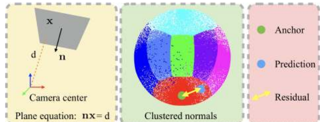
Figure 3. A 3D point x on the plane follows the equation nx = d . We estimate a plane normal n by first picking one of the 7 anchor normals and then regressing the residual 3D vector. Anchor normals are defined by running the K-means clustering algorithm on the ground-truth plane normal vectors.
