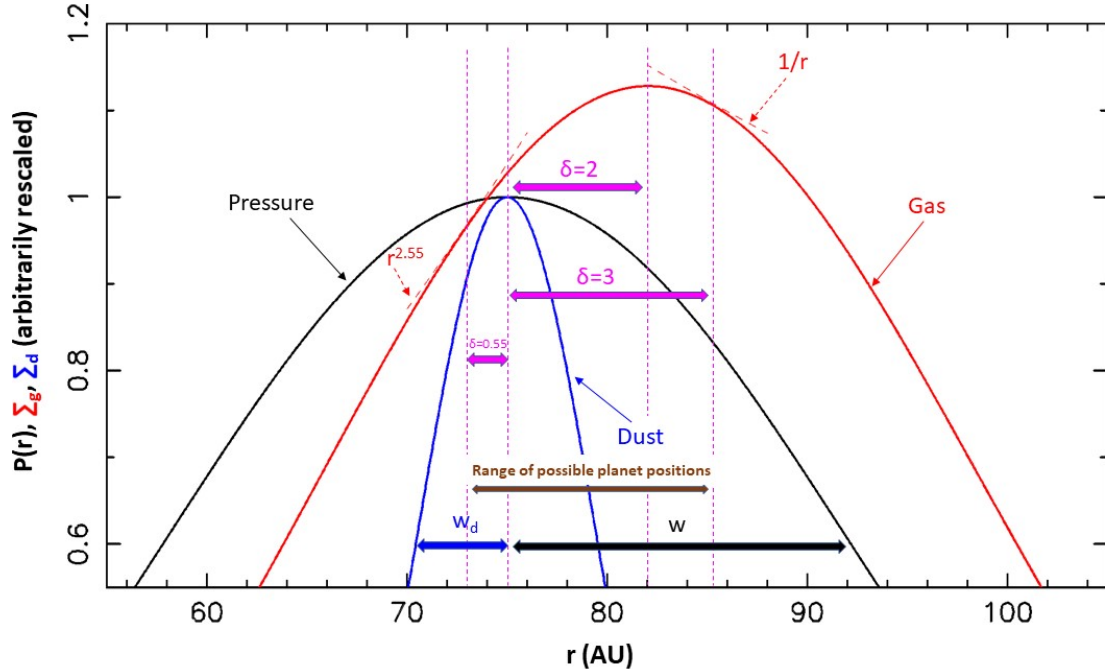
Fig. 1. Radial profiles of pressure (black), gas surface density (red), and dust surface density (blue) for the DHSARP ring B77, from Dullemond et al. (2018) – see Sect. 3. The vertical scale of each profile has been renormalized for illustrative purposes. The dashed thin red curves show the profiles r^{-2.55} and 1/r , and their tangential points to the red solid curve shows the locations where the gas surface density profile has locally these profiles. These two locations delimit the range of possible positions of the planet at the migration trap, depending on the degree of saturation of the vortensity-driven corotation torque. Their distances relative to the location of the pressure maximum are given in terms of the parameter \delta , as well as the location of the maximum of the gas surface-density distribution. The widths w and w_d in Eqs. (1) and (4) are also graphically represented.
