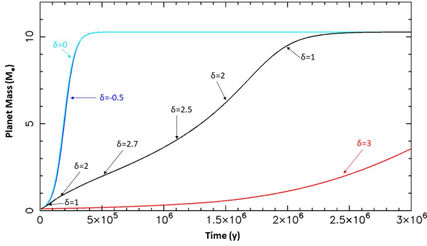
Fig. 3. Same as Fig. 2, but rescaling the geometry of the B77 DHSARP ring at 5 AU and increasing the dust surface density \propto 1/r^{3/2} .
