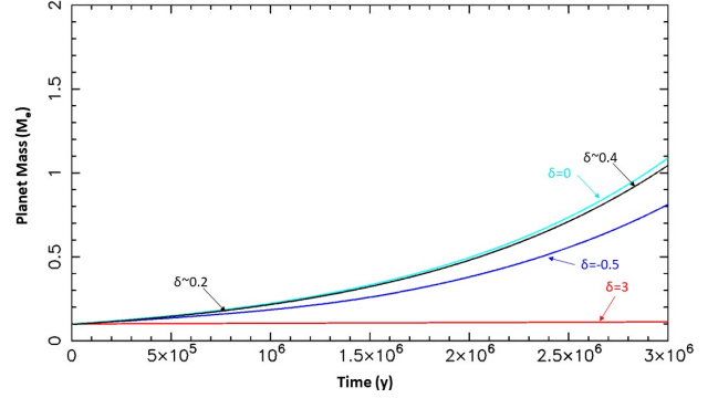
Fig. 2. Evolution of the mass of a planet of initially 0.1 M_{\oplus} accreting pebbles in the B77 DSHARP ring, for three different locations (i.e., values of \delta ) relative to the position of the pressure maximum as well as a case (black curve) where the planet follows the (mass-dependent) location of the planet trap as it grows, and therefore \delta changes with time (from \sim 0.2 to \sim 0.4 ).
