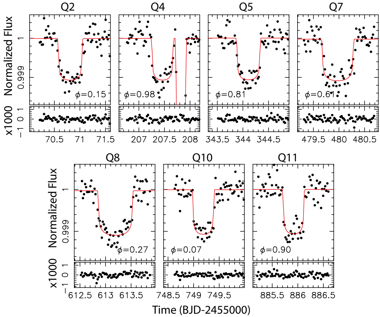
Fig. 14.— Photometric-dynamical model fit to individual planet transits. In Quarter 4 (Q4), the planet transit occurs just before a primary eclipse.
