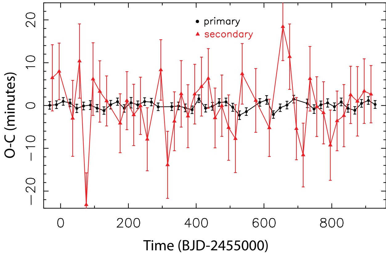
Fig. 3.— O-C offsets measured for the primary and secondary (red in the online version) eclipses of KIC 4862625.
