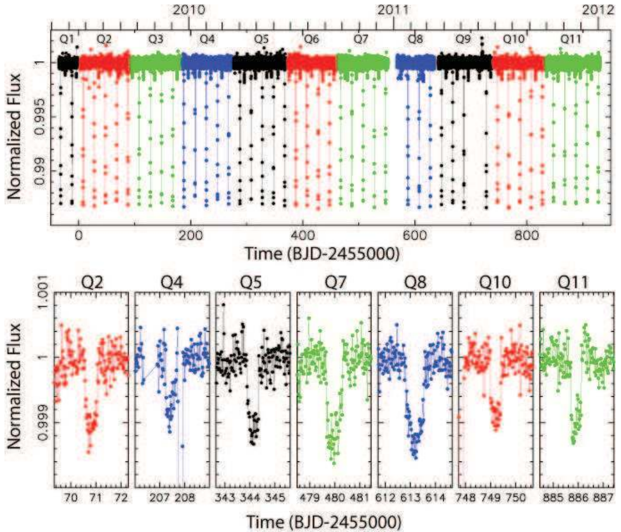
Fig. 2.— Top: Normalized Kepler light curve for KIC 4862625 for Quarters 1-11 Bottom: Individual transits of the planet across star Aa identified in Quarters 1-11. In Quarter 4 (Q4), the planet transit occurs just before a primary eclipse.
