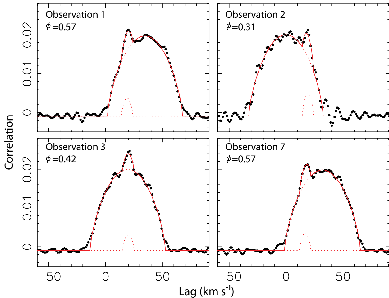
Fig. 7.— The Broadening functions and the analytic broadening kernel fits (solid line for the sum, dotted lines for each component separately) for a subset of the Keck HIRES radial velocity observations taken at different binary orbital phases ( \phi ).
