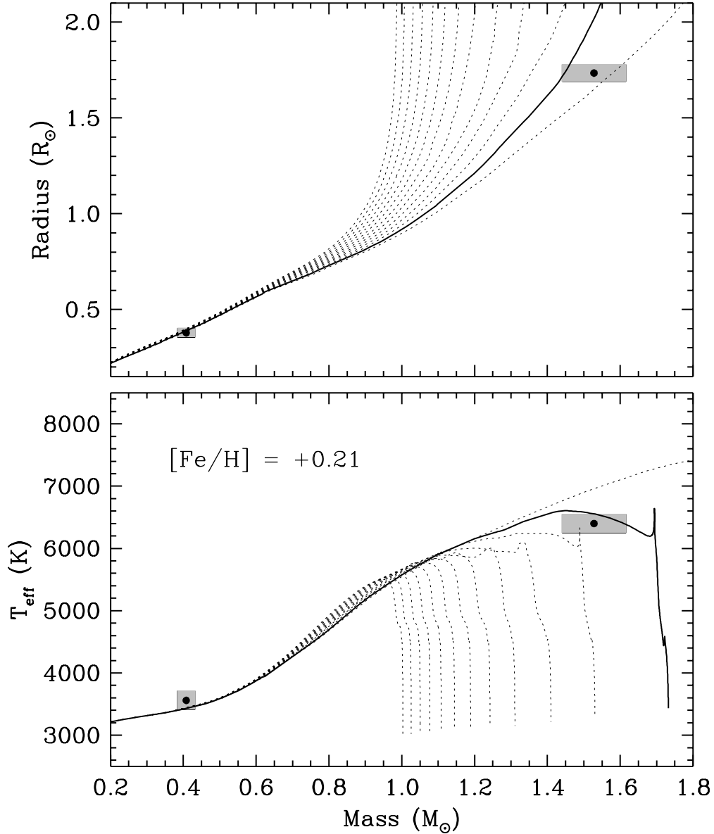
Fig. 12.— Mass, radius, and effective temperatures for Aa and Ab compared against 1–13 Gyr model isochrones from the Dartmouth series by Dotter et al. (2008) , for the measured metallicity of the system ( [\text{Fe}/\text{H}] = +0.21 \pm 0.08 ). The solid line corresponds to a 2 Gyr isochrone, for reference. (Top) Mass–radius diagram showing good agreement for both stars (Aa and Ab) for an age between 1 and 2 Gyr; (Bottom) Mass–temperature diagram again showing that the models match our estimated temperatures, within the errors.
