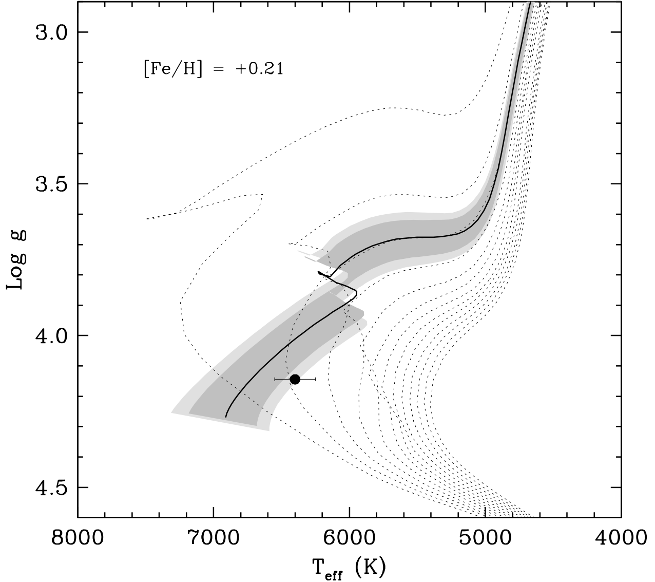
Fig. 11.— Stellar evolution models from the Y 2 (Yonsei-Yale) series by Yi et al. (2001) compared against the measurements for the Aa. The solid line represents an evolutionary track for the measured mass ( M_{\text{Aa}} = 1.528 \pm 0.087 M_{\odot} ) and metallicity ( [\text{Fe}/\text{H}] = +0.21 \pm 0.08 ), and the dotted lines are 1–13 Gyr isochrones (left to right) in steps of 1 Gyr. The uncertainty in the location of the track that comes from the observational errors is shown by the shaded area. The darker area reflects the mass error, and the lighter area includes also the uncertainty in the metallicity.
