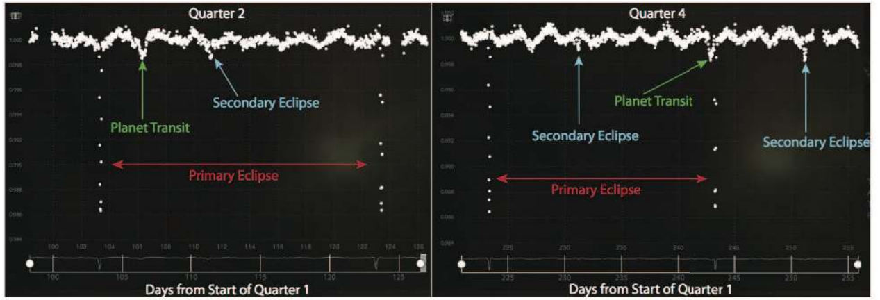
Fig. 1.— Planetary transits in addition to binary-star eclipses identified by Planet Hunters volunteers in KIC 4862625 as viewed in the Planet Hunters interface.
