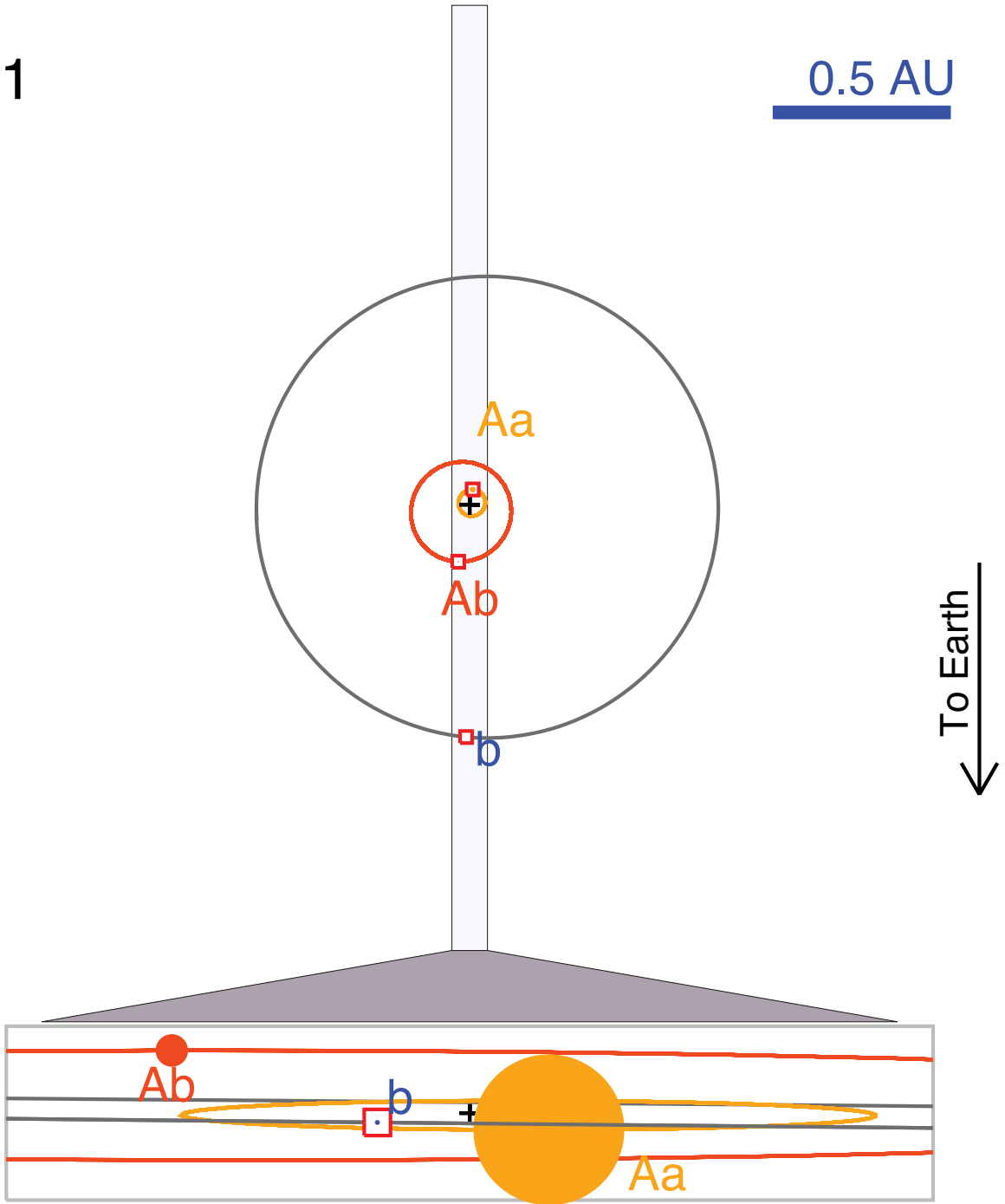
Fig. 13.— Orbital configuration of the PH1 system for the reference epoch, t_0 = 2,454,970 (BJD). The inner close binary (primary star Aa and the secondary star Ab) and the planet (labeled b) are shown. The outer visual binary (Ba and Bb) is not depicted. Top: A scaled, face-on view of the orbits. On this scale the stars and the planet are too small to be seen, and their positions are represented by the boxes. Bottom: The region between the vertical lines in the top diagram is shown on an expanded scale with an orientation corresponding to what would be seen from Earth.
