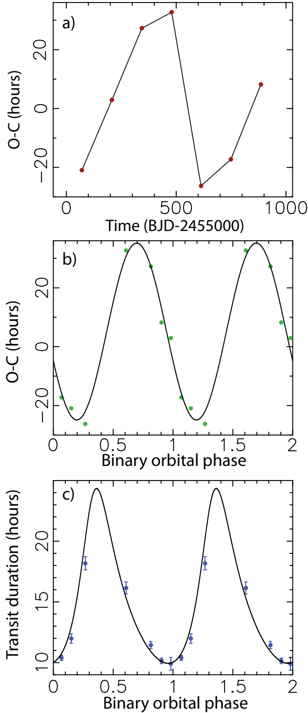
Fig. 4.— O-C offsets and transit durations for the circumbinary planet. a) O-C offsets measured for the planet transits versus time. The 1\text{-}\sigma error bars are plotted. With uncertainties on the transit times on the order of \sim 5 minutes, the error bars are smaller than the size of the symbol. b) O-C offsets measured for the planet transits versus binary orbital phase. The 1\text{-}\sigma error bars are plotted. With uncertainties on the transit times on the order of \sim 5 minutes, the error bars are smaller than the size of the symbol. c) Transit duration as a function of binary orbital phase. Transits near secondary eclipse \phi = 0.39 are wider than those close to primary eclipse \phi = 0.0
