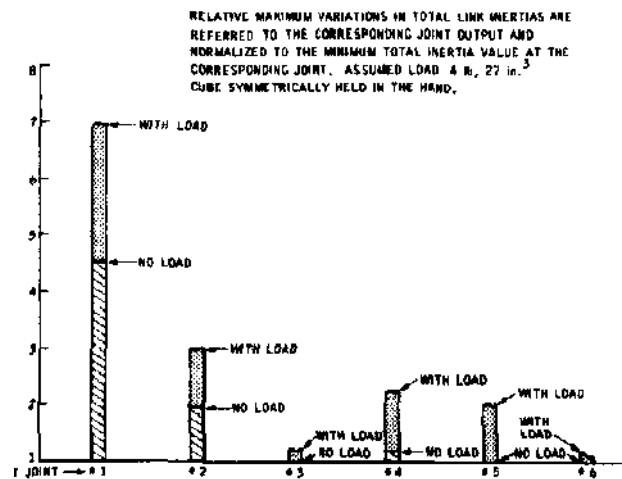
Fig. 9. Relative Maximum Variations In Total Link Inertias
