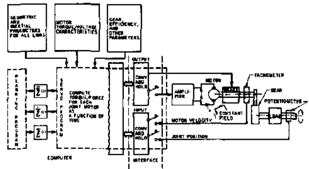
Fig. 8. Manipulator Servo Scheme
