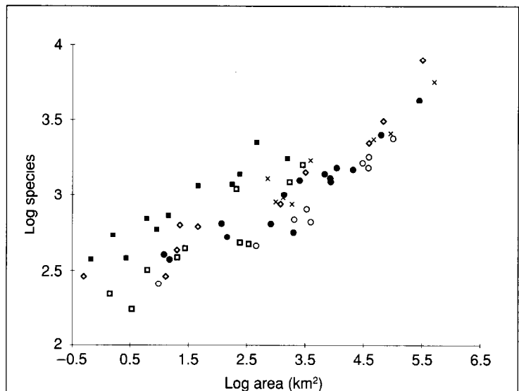
Fig. 2. Species-area curves and regressions from mediterranean-climate regions. Diamonds, SW Australia; filled squares, Cape (SW); unfilled squares, Cape (SE); crosses, Mediterranean Basin; unfilled circles, Chile; filled circles, California. Mediterranean Basin data are from the Iberian Peninsula. All slopes are homogeneous but intercepts ( k -values) vary. Relative diversities of the different regions (see text) are ratios of their respective k -values. Data from Refs 3, 15 and 41.
