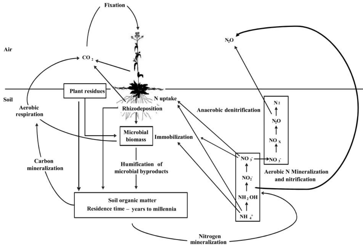
FIG. 1. Hypothetical model illustrating factors affecting \text{CO}_2 and \text{N}_2\text{O} emission from soil and the role of plants in controlling emissions of these gases through their influence on microbial biomass increment in soil by organic matter input (plant residues and rhizodeposits.)
