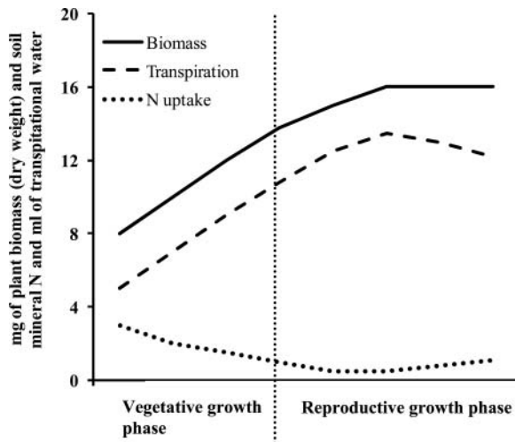
FIG. 3. Hypothetical graph illustrating the pattern of transpiration (ml) and concentration of mineral N from soil ( \text{mg kg}^{-1} of dry soil) with increasing plant biomass (mg of dry weight) under controlled conditions. Rate of transpiration increases with increasing plant biomass and therefore is higher at reproductive growth phase. The concentration of mineral N of soil decreases with increasing plant biomass and therefore, it's concentration is higher in soil at the vegetative growth phase of plant.
