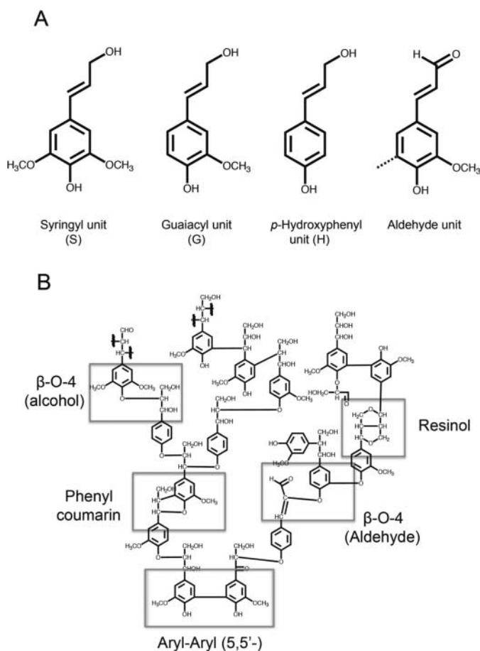
FIG. 8. (a) Phenolic alcohols (syringyl, guaiacyl and hydroxyphenyl alcohol) and phenolic aldehyde precursor units (monolignols) of lignin polymer and (b) and linkages between units; a phenylcoumaran linkage between guaiacyl alcohol units, a \beta -O-4 linkage between normal alcohol units, \beta -O-4 linkage between aldehyde units and a resinol linkage found in P -hydroxyphenyl lignin (Talbot et al. , 2012).
