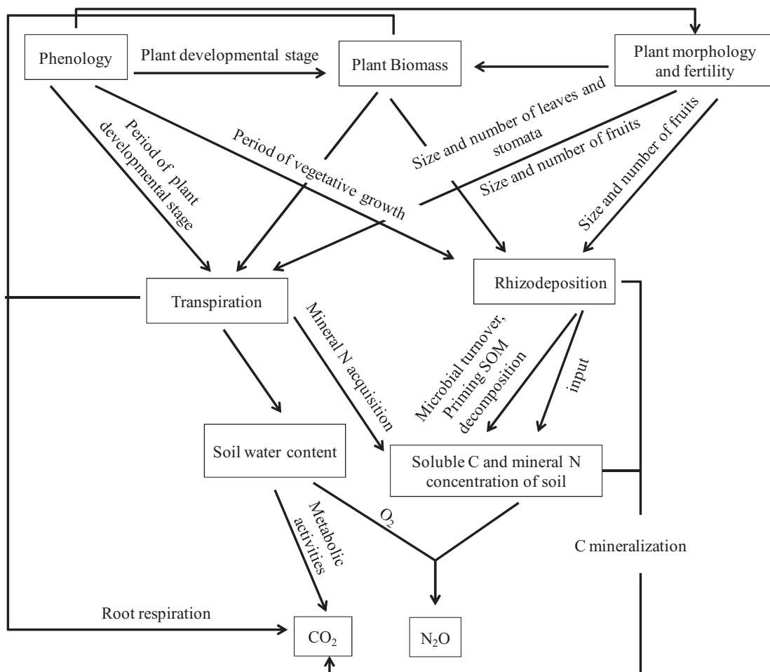
FIG. 2. Hypothetical model illustrating the role of morphological and phenological traits of A. thaliana cell wall mutants upon CO 2 and N 2 O emission from soil. Plant phenology, morphology and plant fertility influence emissions of CO 2 and N 2 O via water contents, amount of mineral N and rhizodeposits of soil.
