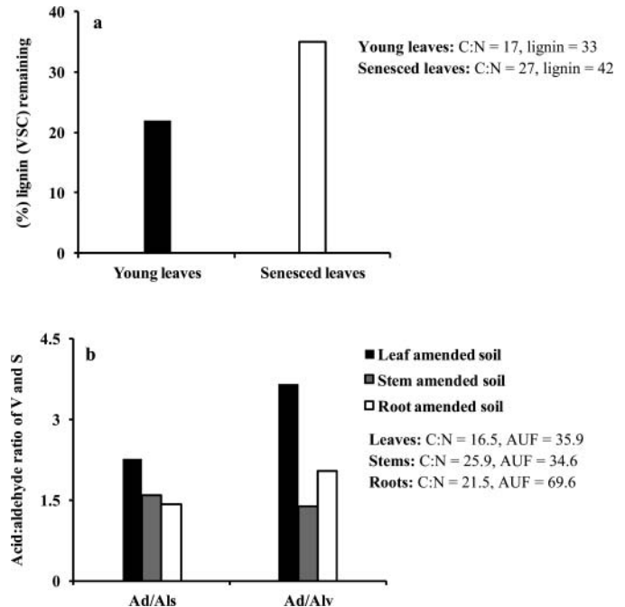
FIG. 9. (a) Influence of C:N ratio and lignin concentration (total of VSC) of young and senesced leaves of Festuca arundinacea on lignin degradation after 44 weeks of burial in soil in litter bags (Sanaullah et al. , 2010) young leaves that had lower C:N ratio and lower concentration of lignin resulted in higher degradation of lignin in soil (b) influence of residue type of corn on lignin degradation of soil (Yanni et al. , 2011) leaves that had a lower C:N ratio and lower concentration of lignin resulted in higher degradation of lignin in soil.
