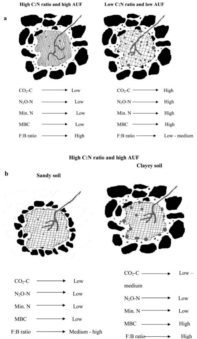
FIG. 10. Conceptual model illustrates (a) the influence of plant residue chemistry (C:N ratio and concentration of acid unhydrolyzable fraction (AUF)) on emission of CO_2 -C, N_2O -N, concentration of mineral N (min. N), microbial biomass C (MBC), and fungal:bacterial (F:B) ratio within a macro-aggregate (cross section) after incubation period of 63 d, and (b) the interactive effect of texture of soil and chemistry of plant residue on emission of CO_2 -C, N_2O -N, concentration of mineral N, microbial biomass C (MBC), and fungal:bacterial (F:B) ratio within macro-aggregates (cross section) after incubation period of
