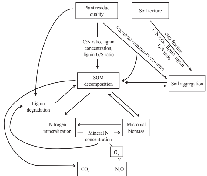
FIG. 6. Hypothetical model illustrating the role of lignin concentration and C:N ratio of plant residue upon soil processes i.e. soil aggregation, SOM decomposition, emission of \text{CO}_2 and \text{N}_2\text{O} , nitrogen mineralization, degradation of lignin and microbial biomass.
