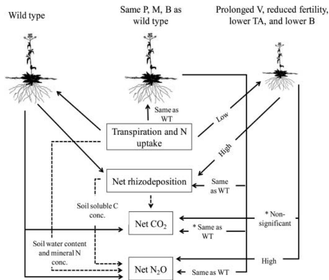
FIG. 5. Hypothetical model illustrating the role of GM cell wall mutants in influencing \text{CO}_2 and \text{N}_2\text{O} emission via their phenological and morphological traits. P is phenology, M morphology, B biomass, V vegetative growth period, TA transpiration apparatus (leaf number and leaf area). Dashed lines represent relationship of factors. * \text{CO}_2 emission from soil is the function of root and microbial respiration, which can be influenced by plant biomass, fertility, and rhizodeposition.
