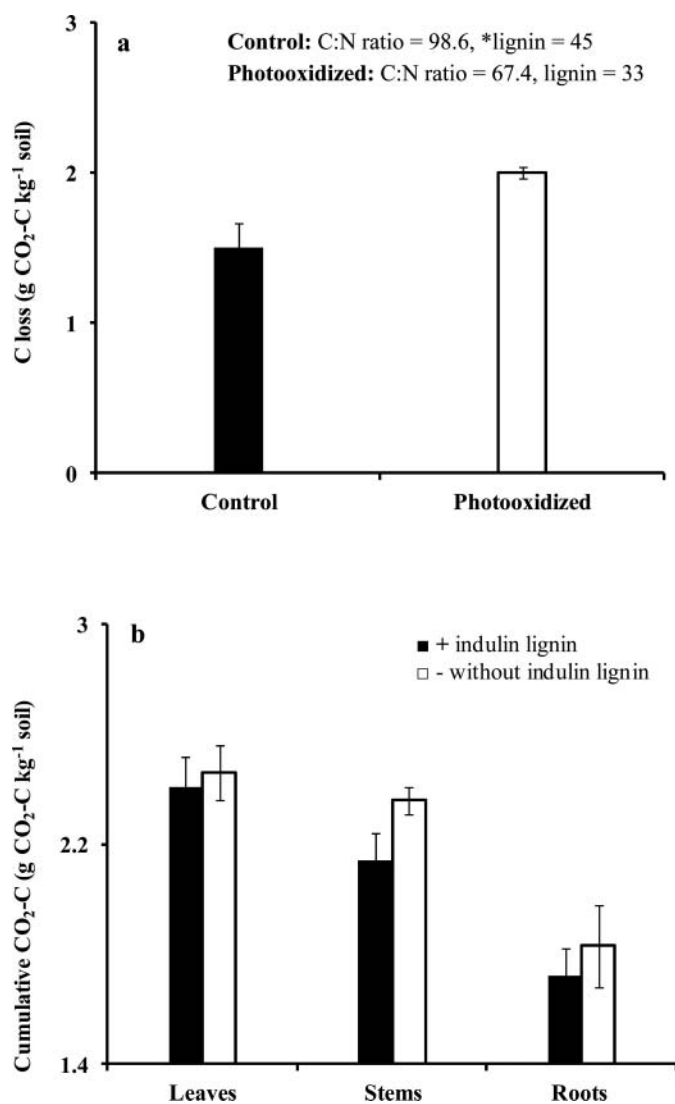
FIG. 7. (a) Influence of photooxidized residue of Calamagrostis epigios on C loss (measured as CO 2 -C loss g -1 soil) * lignin as cumulative of 2 methoxy 4 vinylphenol and 3,4-dimethoxybenzaldehyde (Frouz et al. , 2011). Significant ~27% reduction in concentration of lignin from photooxidation resulted in ~25% increase in C loss from soil (b) influence of indulin lignin mixed with plant residue type on CO 2 -C production from soil (Yanni et al. , 2011) indulin lignin significantly reduced emission of CO 2 from soil amended with stem residue.
