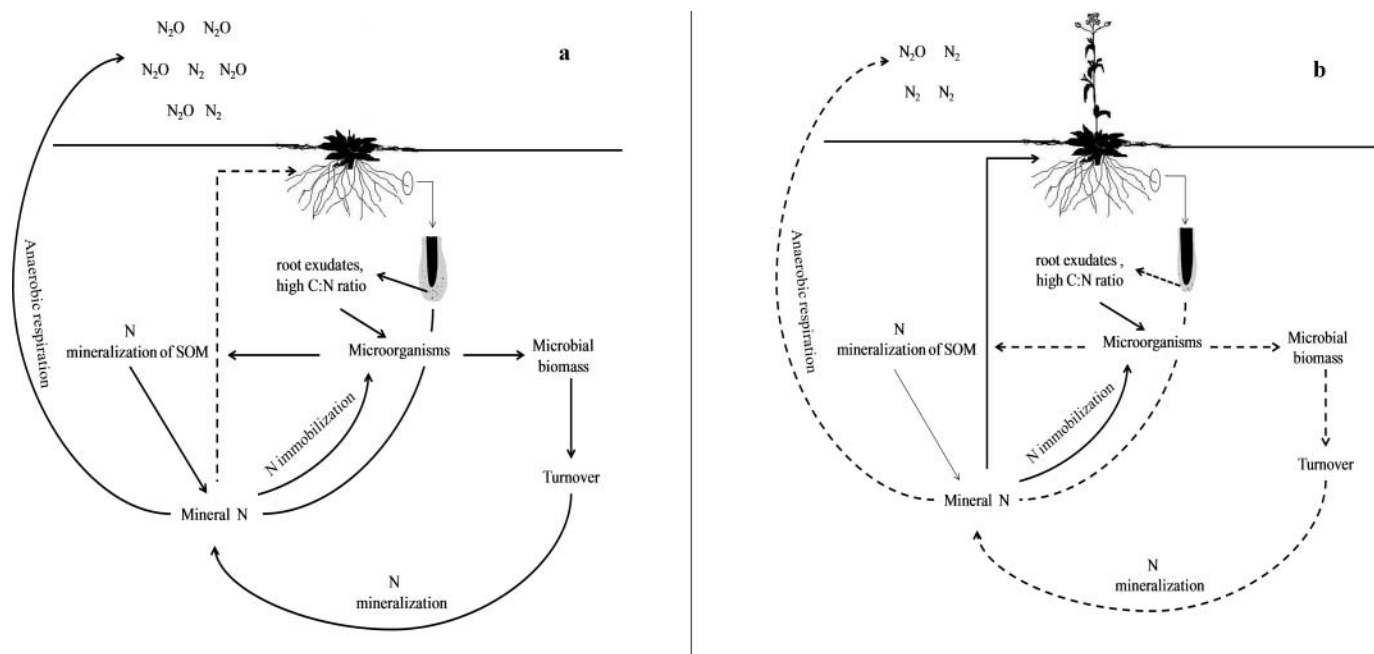
FIG. 4. Hypothetical model illustrating the influence of rhizodeposition at vegetative (a) and reproductive (b) phase on processes leading to emission of N_2O from soil. Plain and dashed lines indicate respectively the strong and weak intensities of related processes. At the vegetative growth phase, the greater amount of rhizodeposits in soil enhances microbial mediated mineralization of N via rhizodeposit-driven higher microbial biomass. In return, the higher microbial biomass and higher amount of mineral N in concert with organic C source (rhizodeposition) in soil causes higher emission of N_2O in anaerobic conditions.
