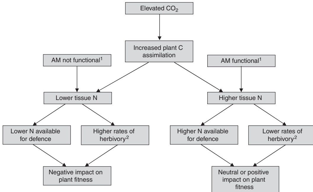
Fig. 3. Hypothesised links between eCO 2 , plant (C 3 ) N nutrition, AM and plant defences. (1) AM function in this example refers to increased nutrient uptake and delivery to the plant. (2) Decreased tissue N leads to increased rates of herbivory as herbivores consume more plant tissue to satisfy their dietary N requirements.
