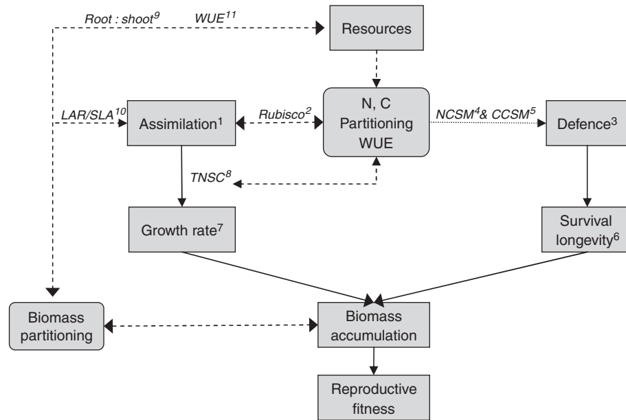
Fig. 2. Resource allocation within plants. Plant morphology, biochemistry and the efficiency of the physiological processes are integrated with nutrient supply and partitioning. Any change in resource supply or resource-use efficiency affects the partitioning of resources and the defence–growth equilibrium. (1) Assimilation rate is controlled by the size and effectiveness of the photosynthetic machinery, especially (2) Rubisco, as it accounts for ~25% of leaf N. A smaller but variable proportion of resources are allocated to the (3) synthesis of (C- or N-based) defensive secondary compounds, here classified on whether they contain (4) nitrogen (NCSM) or (5) not (CCSM). (6) Defended plants are assumed to have greater longevity, but at the cost of (7) high growth rates. (8) Plants grown at elevated atmospheric [CO 2 ] accumulate more total non-structural carbohydrates, which inhibit Rubisco synthesis. Low nutrient supply and elevated atmospheric [CO 2 ] is associated with (9) greater root growth (root : shoot ratio), and (10) decreased leaf area ratio and specific leaf area. (11) These, in turn, affect the ability of plants to acquire water and transpiration rates (WUE).
