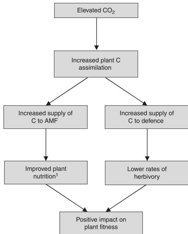
Fig. 4. Hypothesised links between eCO 2 , C assimilation, AM and (C 3 ) plant defences. (1) AM function in this example refers to increased nutrient uptake and delivery to the plant.
