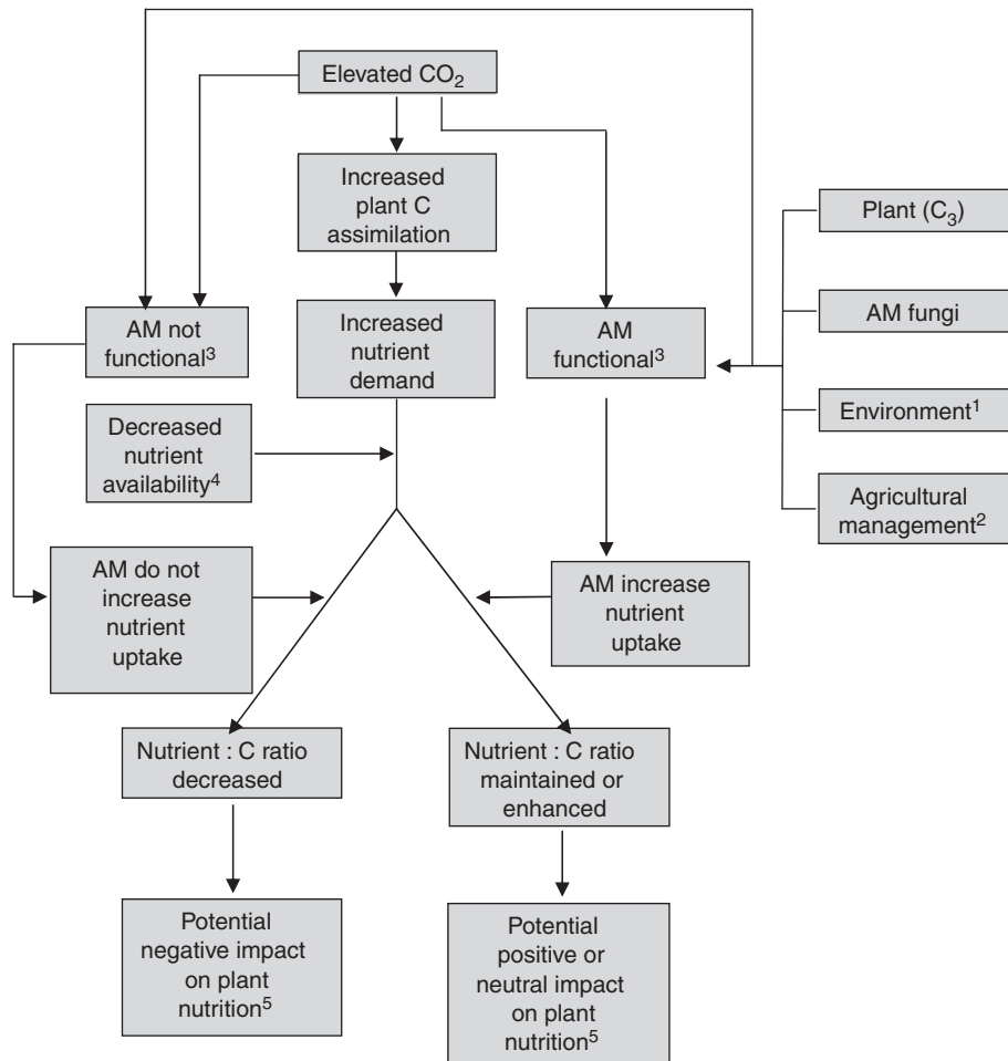
Fig. 1. Potential links between e\text{CO}_2 , agricultural management, AM and plant nutrient acquisition. NB: Emphasis is on nutrient uptake and supply to ( \text{C}_3 ) plants, not C supply to the fungi. (1) Environmental factors aside from e\text{CO}_2 , e.g. edaphic, temperature, etc. (2) Tillage, nutrient management, crop rotations (including fallow). (3) AM function in this example refers to increased nutrient uptake and delivery to the plant. (4) Looming P shortage, limited access due to increased cost. (5) Impact on crop yields, nutrient content or both.
