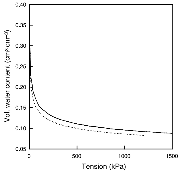
Fig. 6 Moisture release curve for Bullionfield soil with pure water, calculated using van Genuchten's (1980) equation fitted to the experimental data obtained from tension table and pressure plate experiments (solid line). The moisture release curve calculated from the same water contents plotted at 65% of the suction is also shown (dotted line).
