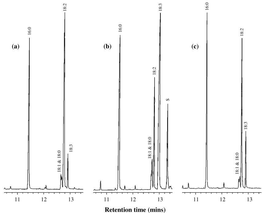
Fig. 1 Gas chromatograms showing the fatty acid composition of the root tissues of: (a) maize (b) lupin and (c) wheat, following extraction, hydrolysis and methyl esterification. Five fatty acids were typically present: saturated (16 : 0 and 18 : 0) and unsaturated (18 : 1, 18 : 2 and 18 : 3). The peak labelled 'S' is due to a 19 : 0 standard which was occasionally added prior to derivatisation.
