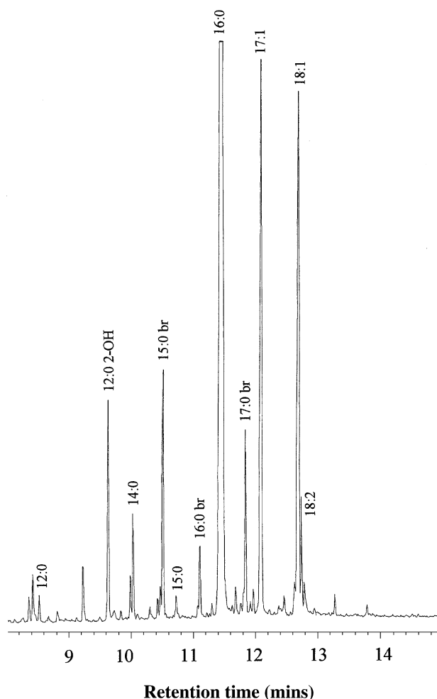
Fig. 4 Fatty acid analysis of a wheat mucilage sample showing clear signs of bacterial contamination. The profile is intense relative to the mucilage chromatograms (i.e. the quantity of fatty acids in the sample is much greater) and consists of fatty acids with odd-numbered carbon chain lengths, branched chains ('br') and occasionally hydroxyl-substitution (12:0 2-OH), in addition to the even-numbered, unbranched fatty acids characteristic of plants.
