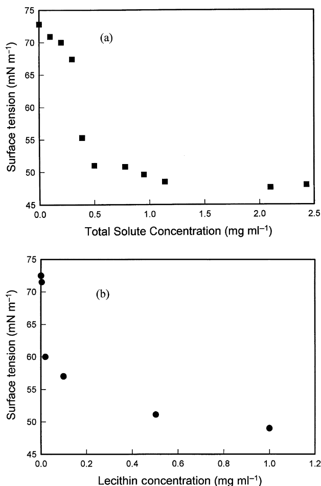
Fig. 3 Variation of surface tension (at 20°C) of (a) filtered wheat mucilage, and (b) soybean lecithin (a phosphatidylcholine), in aqueous solution.
