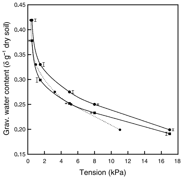
Fig. 5 Water release curves for Bullionfield soil at a density of 1.1 \text{ Mg m}^{-3} with pure water (circles, solid line) and with lecithin solution at a concentration of 500 \text{ mg l}^{-1} (squares, solid line), measured on tension tables. Error bars, offset from the data points for clarity, represent one standard error. For comparison, a moisture release curve calculated from the water content of Bullionfield soil with pure water, but plotted at 65% of the tension, is also shown (circles, dotted line).
