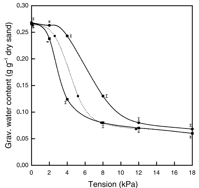
Fig. 7 Water release curves for acid-washed sand at a density of 1.7 \text{ Mg m}^{-3} with pure water (circles, solid line) and with lecithin solution at a concentration of 500 \text{ mg l}^{-1} (squares, solid line), measured on tension tables. Error bars, offset from the data points for clarity, represent one standard error. For comparison, a moisture release curve calculated from the water content of Bullionfield soil with pure water, but plotted at 65% of the tension, is also shown (circles, dotted line).
