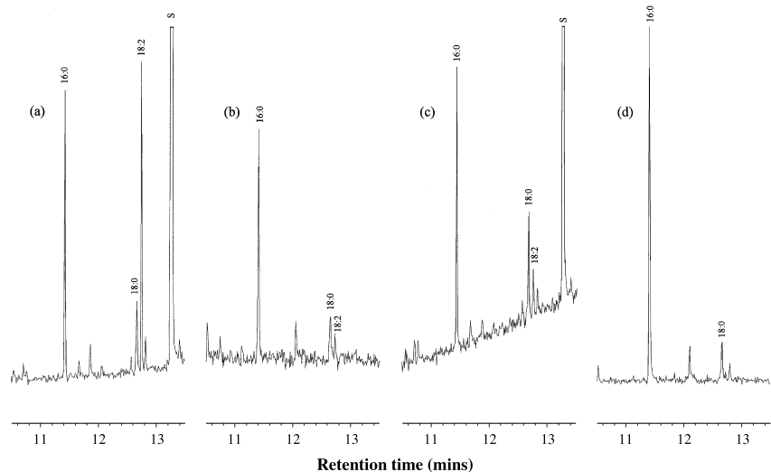
Fig. 2 Gas chromatograms showing the fatty acid composition of: (a) unfiltered maize mucilage; (b) maize mucilage after filtration through a 0.45- \mu\text{m} syringe filter to remove all insoluble plant material; (c) filtered lupin mucilage; (d) filtered wheat mucilage; following extraction, hydrolysis and methyl esterification. In the filtered mucilages, the two saturated fatty acids (16 : 0 and 18 : 0) predominate. The peak labelled 'S' is due to a 19 : 0 standard which was occasionally added prior to derivatisation.
