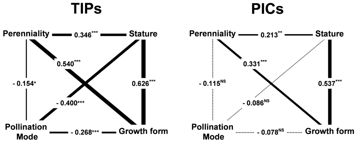
Figure 3 Conventional regressions analyses (TIPs) on the left and phylogenetically-controlled regression analyses (PICs) on the right, among plant traits: growth form, perennality, pollination mode and stature. *** P < 0.001 , ** 0.001 < P < 0.01 , * 0.01 < P < 0.05 and ^{NS} for P > 0.05 .
