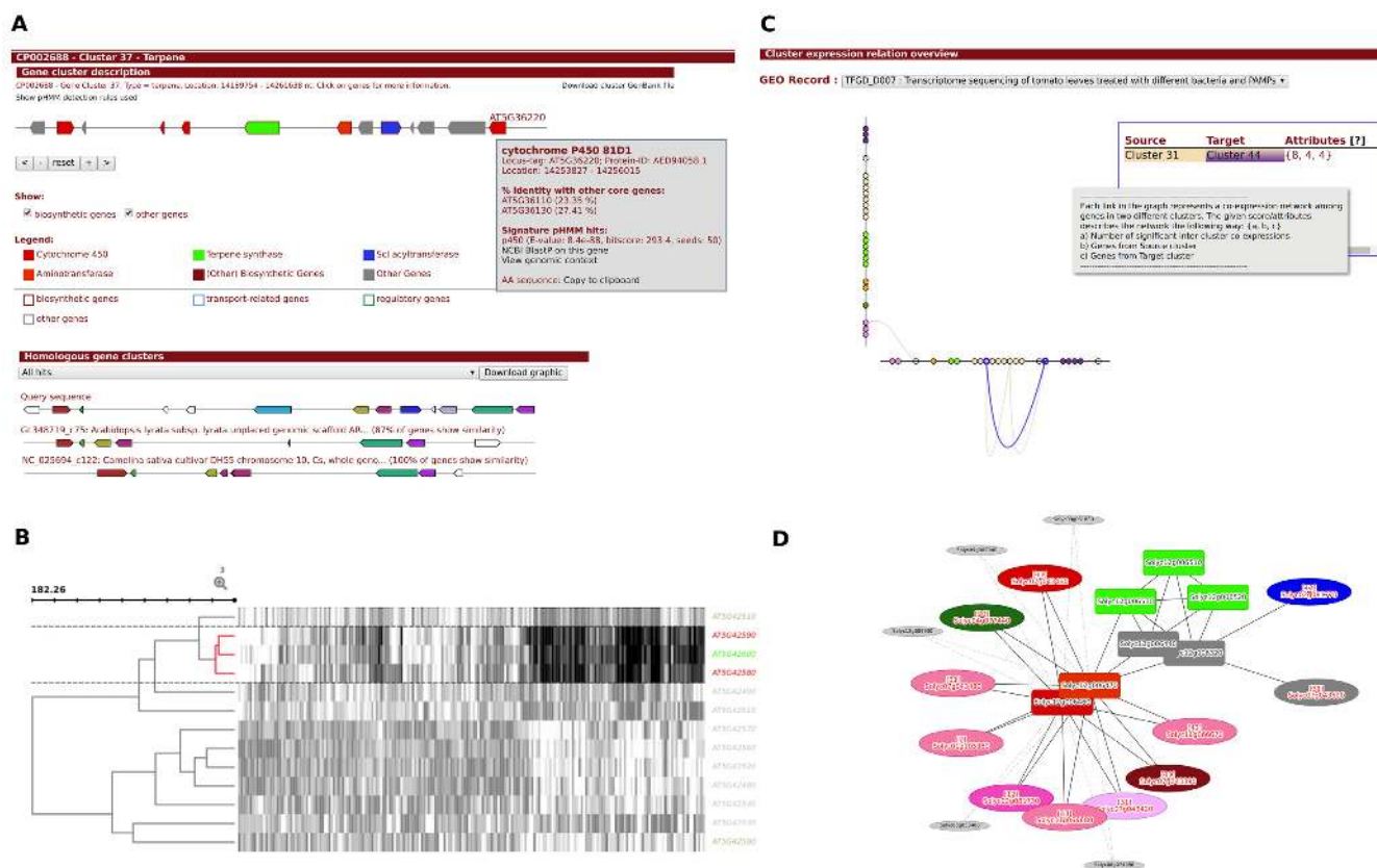
Figure 2. Outputs generated by the plantSMASH pipeline. The figure illustrates several visualized outputs generated by plantSMASH, as they appear for various biosynthetic gene clusters of known natural products. (A) Visual overview generated for each gene cluster; in this case, the tirucalladienol cluster from Arabidopsis thaliana (47) is shown. Gene annotations and pHMM hit details appear on mouse click. Also, ClusterBlast output showing alignment of homologous genomic loci across other genomes of related species is provided. (B) Example of a gene expression heatmap, showing coexpression among the core genes of the marneral BGC from A. thaliana (48) (and not with the flanking genes). (C) Hive plot on the overview page, which highlights pairs of candidate BGCs which show many coexpression correlations between their genes; in this example view, the coexpression links between the two loci encoding \alpha -tomatine biosynthesis in Solanum lycopersicum (20) are highlighted (clusters 31 and 44). (D) Example ego network that summarizes coexpression correlations between members of the \alpha -tomatine gene (cluster 44), as well as with genes in other gene clusters (including the other \alpha -tomatine biosynthetic locus, cluster 31) and with genes elsewhere on the genome.
