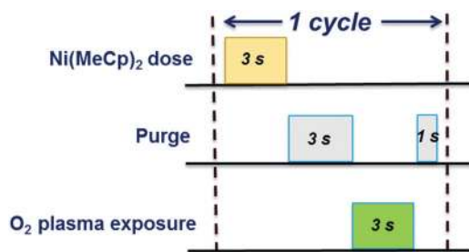
Fig. 1 Schematic of the standard recipe used for plasma-assisted ALD of NiO.
