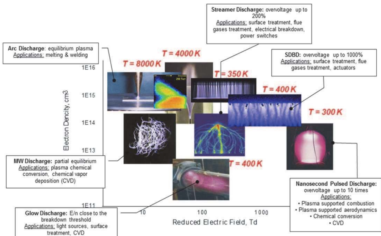
Fig. 18. Discharge development at different overvoltage and plasma generation.
