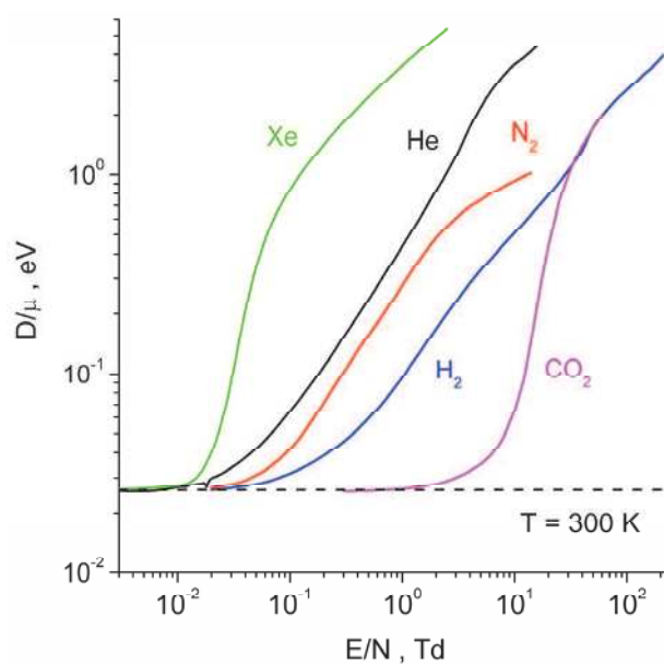
Fig. 15. Characteristic electron energy. He and Ar - [Dutton, 1975]; H 2 , N 2 and CO 2 - [Huxley&Crompton, 1974].
