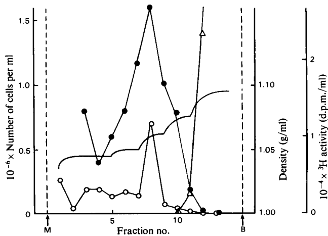
Fig. 3. Separation of rabbit liver cells in a Percoll gradient
