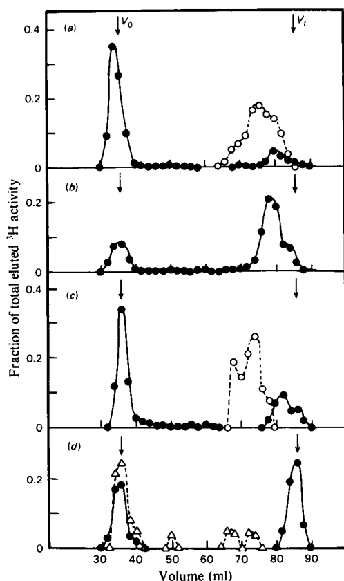
Fig. 2. Gel chromatography of aqueous liver extracts. Samples (1 ml) of the liver extracts described in Table 5 were fractionated on Sephadex G-50 equilibrated with 0.16 M-NaCl/borate (see the Materials and methods section). The chromatograms (●) represent the following times from injection to circulatory arrest: (a) 19 min (expt. 3); (b) 90 min (expt. 1); (c) 4.5 h (expt. 6); (d) 24 h (expt. 8). Aliquots (1 ml) of peak V_0 fractions (expts. 3 and 6) were brought to pH 5.8 with 0.1 ml of 1 M-acetic acid and incubated at 37°C with 200 i.u. of testicular hyaluronidase. After 6 h another 100 i.u. of enzyme was added and incubation was continued for 18 h. The reaction mixture was centrifuged at 1850 g for 40 min, and 1 ml of the supernatant was applied to the same column equilibrated in 0.15 M-NaCl/phosphate (○). The peak V_0 fraction from expt. 8 was incubated at 37°C for 18 h with 100 turbidity-reducing units of Streptomyces hyaluronidase in a final volume of 1.5 ml of 0.16 M-NaCl/borate; 1 ml of this was applied to the column (△). Labelled hyaluronic acid was completely degraded to oligosaccharides under the same conditions (results not shown).
