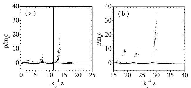
FIG. 2. Longitudinal momentum versus z of the plasma electrons for Figs. 1(a) and 1(b).
