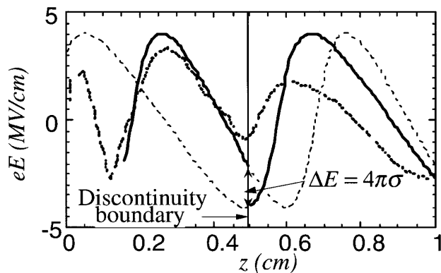
FIG. 3. Plot of the wake electric field in the two regions ( n_0 = 3.5 \times 10^{13} \text{ cm}^{-3} for z > 0.5 \text{ cm} and n_0 = 5 \times 10^{13} \text{ cm}^{-3} for z < 0.5 \text{ cm} ). The solid line indicates the field in the region calculated from the analytical model, while the dashed line indicates the model-derived field in the conjugate region. The thick dotted line is the field calculated from a 1D PIC simulation.
