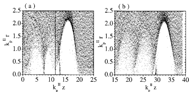
FIG. 1. Configuration space ( r, z ) distributions of the plasma electrons from the MAGIC code 2D PIC simulation.
