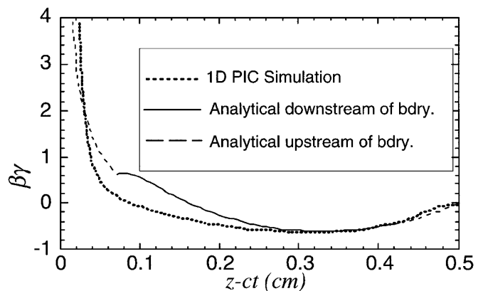
FIG. 4. Phase space trajectory of a trapped electron originating 0.01 cm downstream of the plasma density transition, for the simulation and parameters of Fig. 1.
