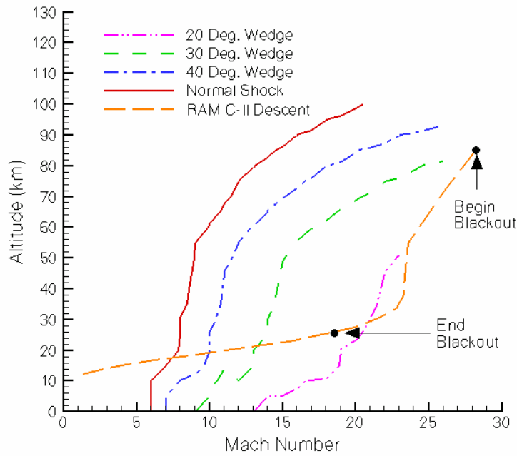
Figure 13: Blackout points along the reentry trajectory (from Ref. 19) for the RAM C-II flight test vehicle along with plasma attenuation coefficient unity lines for various wedge angles.
